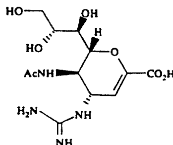
4-guanidino analogue of DANA
