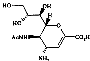
4-amino analogue of DANA
