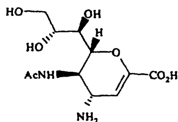
4-amino analogue of DANA
