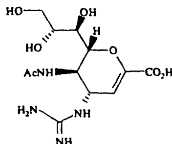
4-guanidino analogue of DANA
