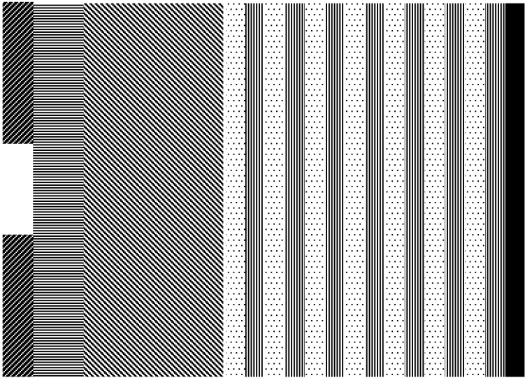
FIG 1 photoresist ARC (anti reflective coating) APF Amorphous carbon mask SiN SiO Si Sidewall passivation layer (FIG 1a)
