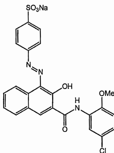
Compound 2
