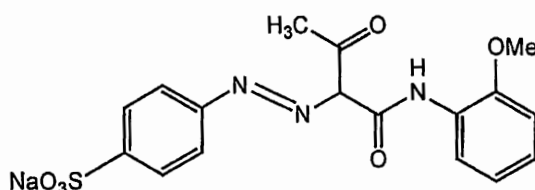
Compound I
