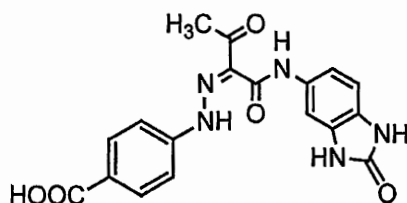
Compound 3
