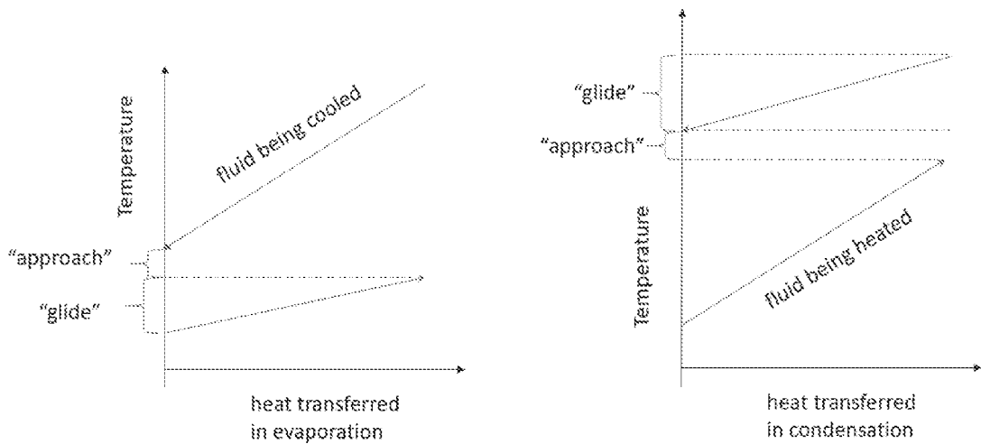
Figure 2 – temperatures in crossflow heat exchangers for non-azeotropic refrigerant
