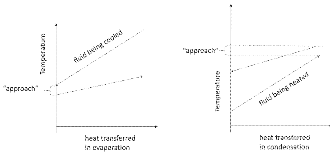
Figure 3 – temperatures in counterflow heat exchangers for non-azeotropic refrigerant
