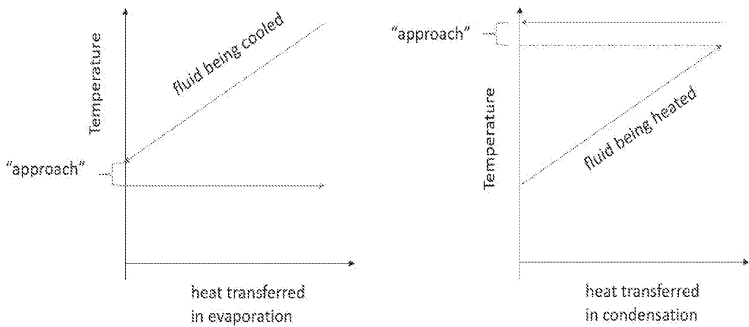
Figure 1 – temperatures in heat exchangers for single refrigerant or azeotropic refrigerant
