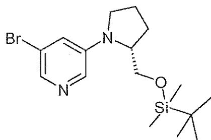
[B] 3-Bromo-5-[(R)-2-( tert -butyl-dimethyl-silanyloxymethyl)-pyrrolidin-1-yl]-pyridine
