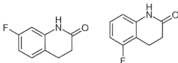
10 (compound A) and (compound B)
