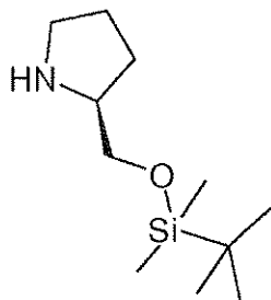
[A] (S)-2-( tert -Butyl-dimethyl-silanyloxymethyl)-pyrrolidine
