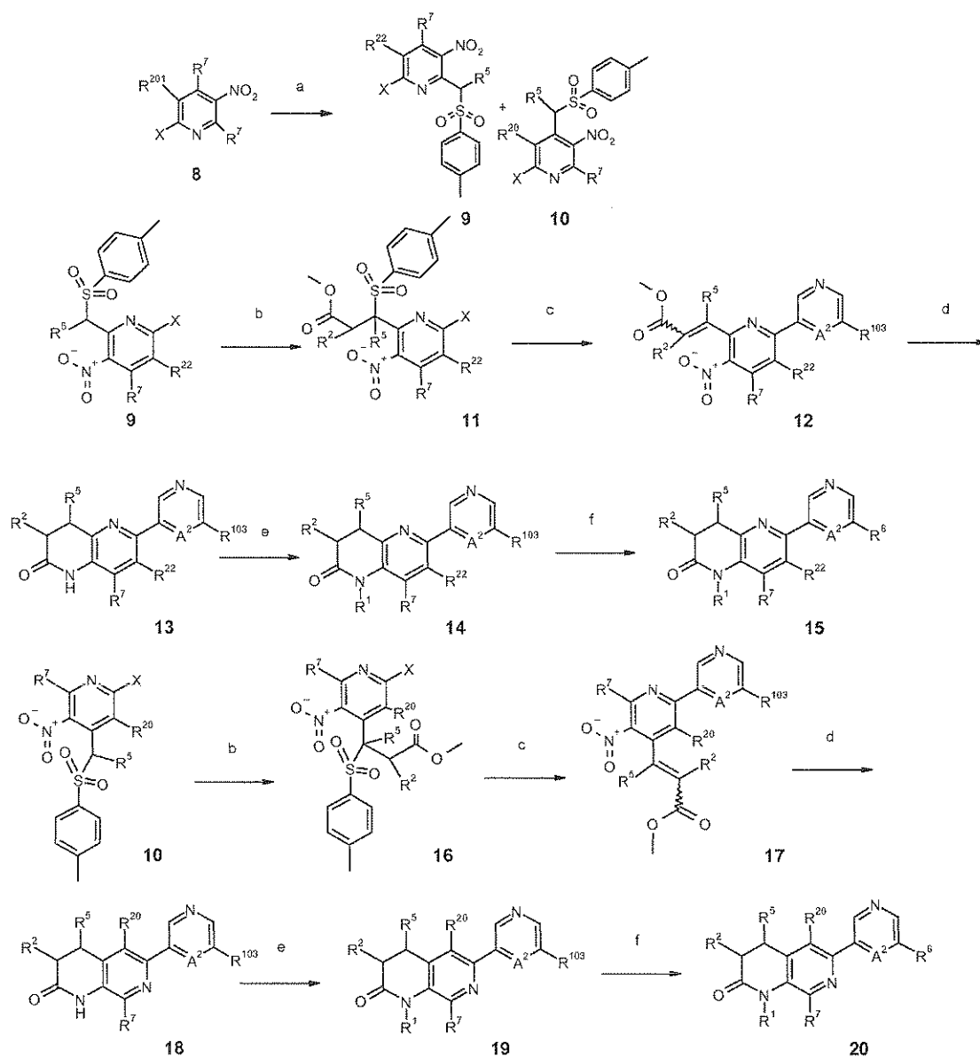
Scheme 1b
