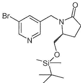
[B] (S)-1-(5-Bromo-pyridin-3-ylmethyl)-5-( tert -butyl-dimethyl-silanyloxymethyl)- pyrrolidin-2-one
