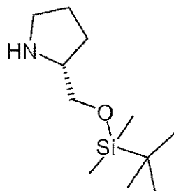
[A] (R)-2-( tert -Butyl-dimethyl-silanyloxymethyl)-pyrrolidine
