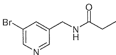
[A] N-(5-Bromo-pyridin-3-ylmethyl)-propionamide
