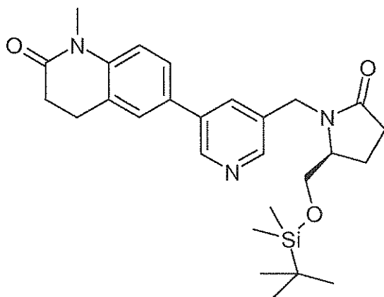
[A] (S)-5-( tert -Butyl-dimethyl-silanyloxymethyl)-pyrrolidin-2-one
