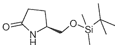
[A] (S)-5-( tert -Butyl-dimethyl-silanyloxymethyl)-pyrrolidin-2-one
