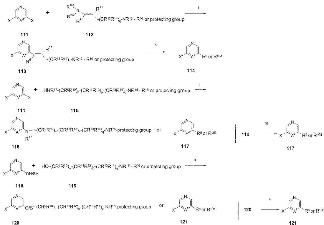
Scheme 2b
