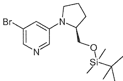
10 [B] 3-Bromo-5-[(S)-2-( tert -butyl-dimethyl-silanyloxymethyl)-pyrrolidin-1-yl]-pyridine
