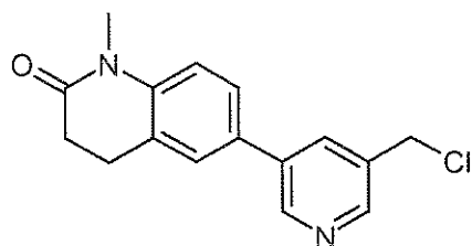
[B] 6-(5-Chloromethyl-pyridin-3-yl)-1-methyl-3,4-dihydro-1 H -quinolin-2-one
