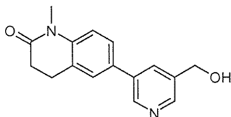
[A] 6-(5-Hydroxymethyl-pyridin-3-yl)-1-methyl-3,4-dihydro-1 H -quinolin-2-one
