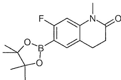
[B] 7-Fluoro-1-methyl-6-(4,4,5,5-tetramethyl-[1,3,2]dioxaborolan-2-yl)-3,4-dihydro-1H-quinolin-2-one
