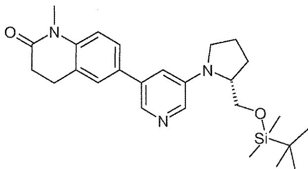
[A] (R)-2-( tert -Butyl-dimethyl-silanyloxymethyl)-pyrrolidine
