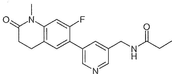
[B] N-[5-(7-Fluoro-1-methyl-2-oxo-1,2,3,4-tetrahydro-quinolin-6-yl)-pyridin-3-ylmethyl]-propionamide
