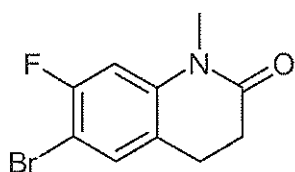
[A] 6-Bromo-7-fluoro-1-methyl-3,4-dihydro-1H-quinolin-2-one
