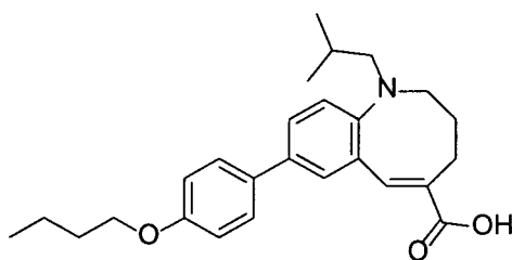
Compound II-OH-C
