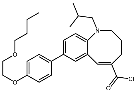
Compound II-Cl
