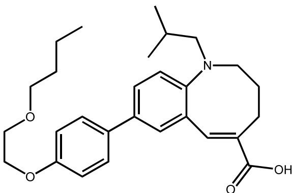
Compound II-OH ;
