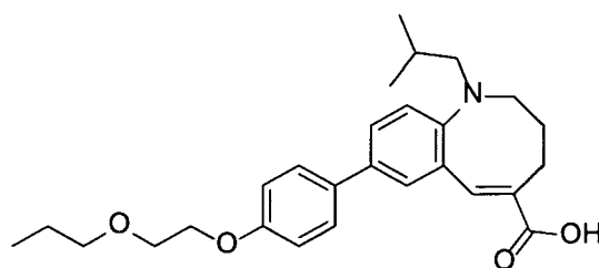
Compound II-OH-B
