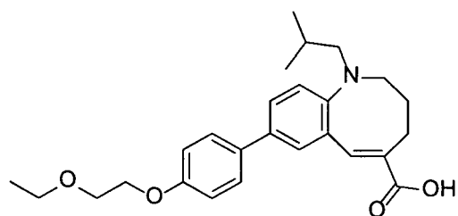
Compound II-OH-A
