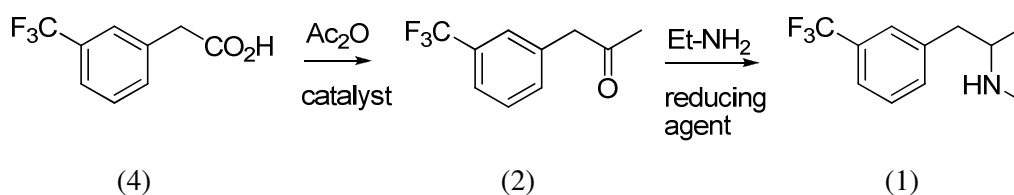
Scheme 4: Preparation of fenfluramine (1) from acid (4) via ketone (2)
