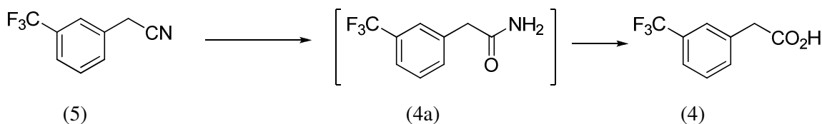
Scheme 5: Hydrolysis of nitrile (5) to acid (4).
