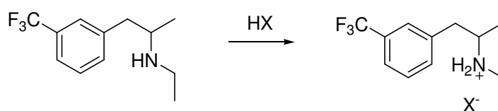
Scheme 8: Preparation of a salt of fenfluramine.
