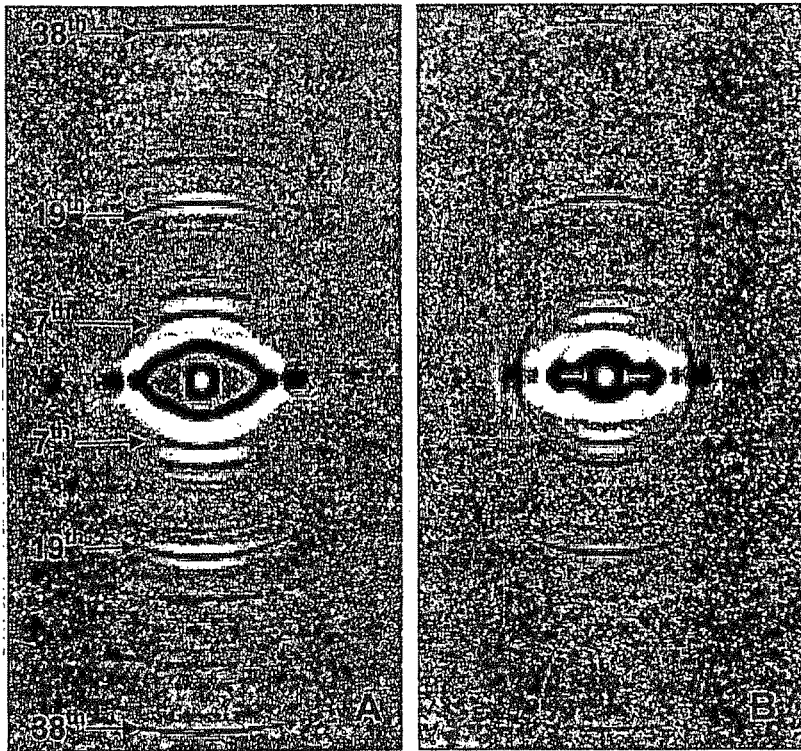
Fig. 6: A: SAXS image of normal hair, showing 7 th , 19 th and 38 th order peaks of the 46.7nm lattice. The data was smoothed using the "Alternative Protocol" described in the text. B: SAXS image of hair from an individual with breast cancer showing a well defined ring in the zone of interest. Note the 7 th , 19 th and 38 th orders are also clearly visible.
