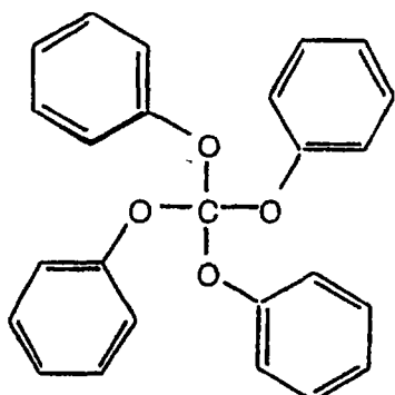
Tetraphenoxy-methane (TPM)
