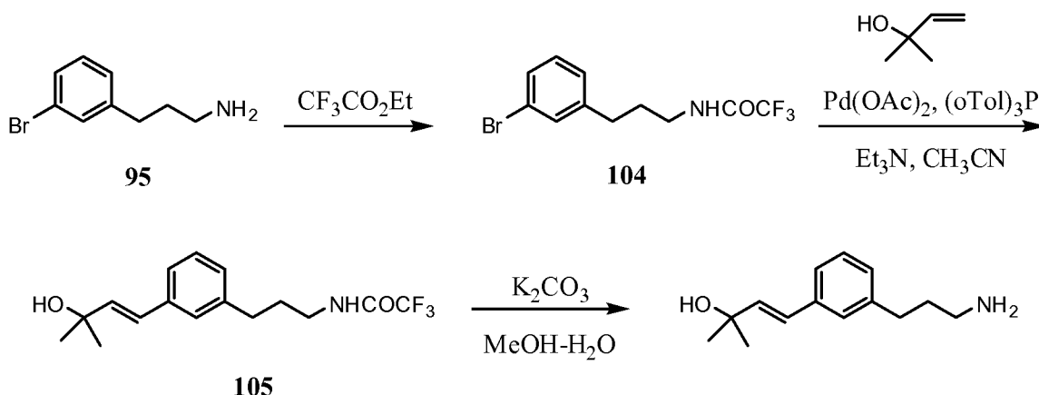
SCHEME 35
