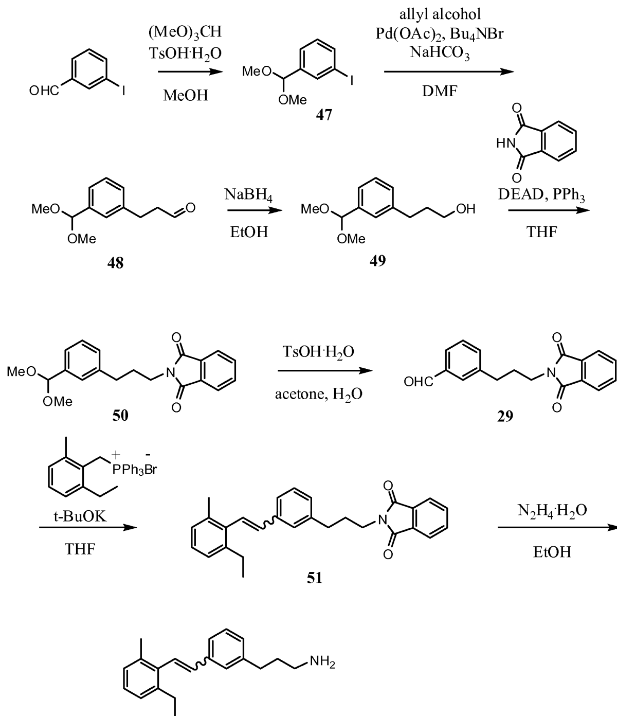
SCHEME 15
