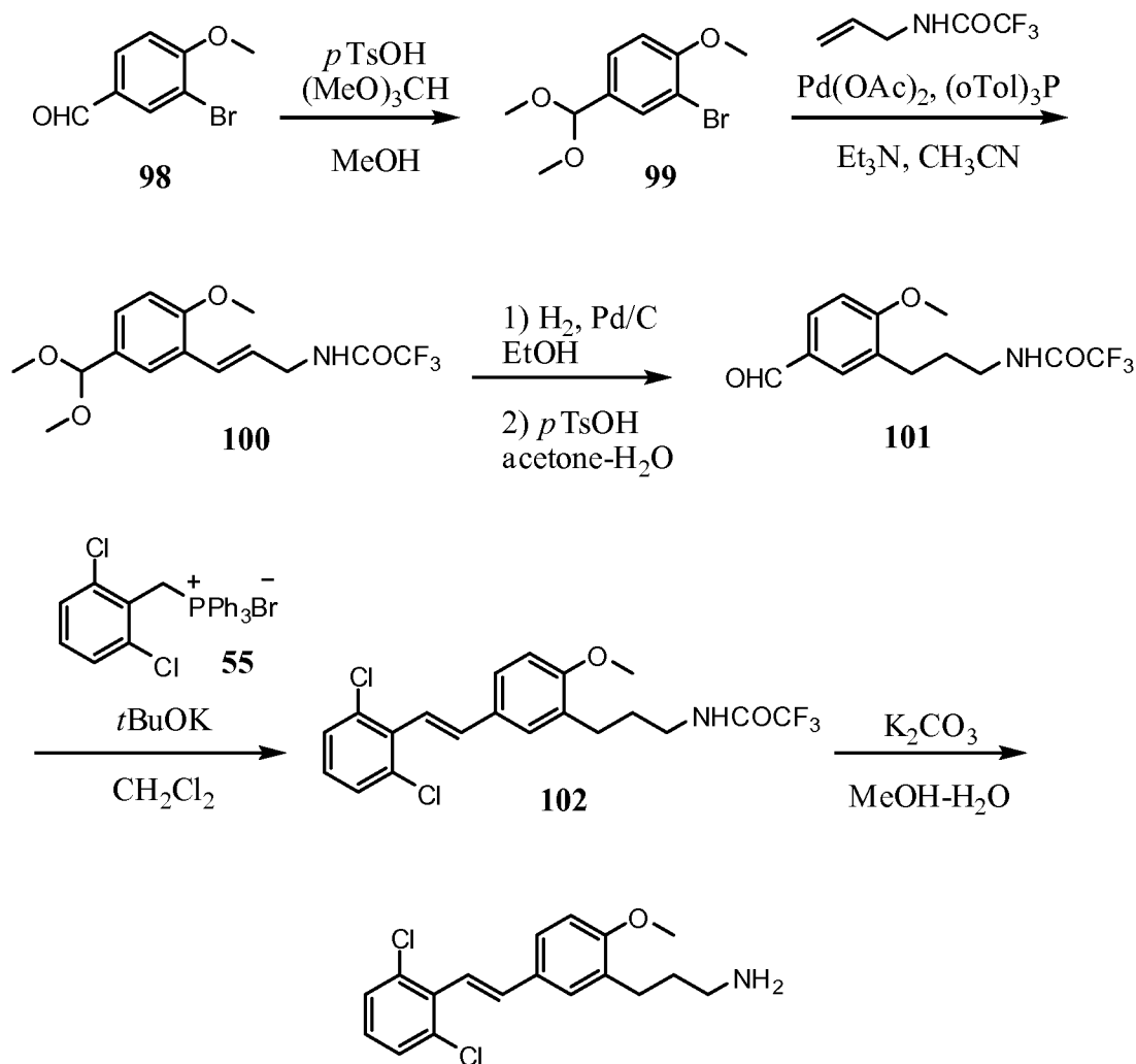
SCHEME 33
