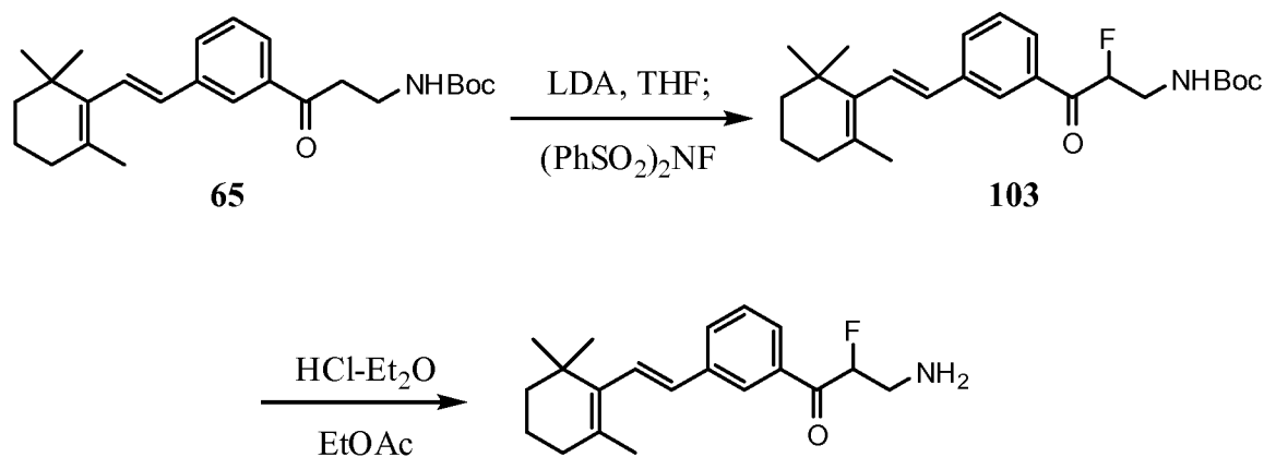
SCHEME 34
