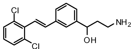
SCHEME 18
