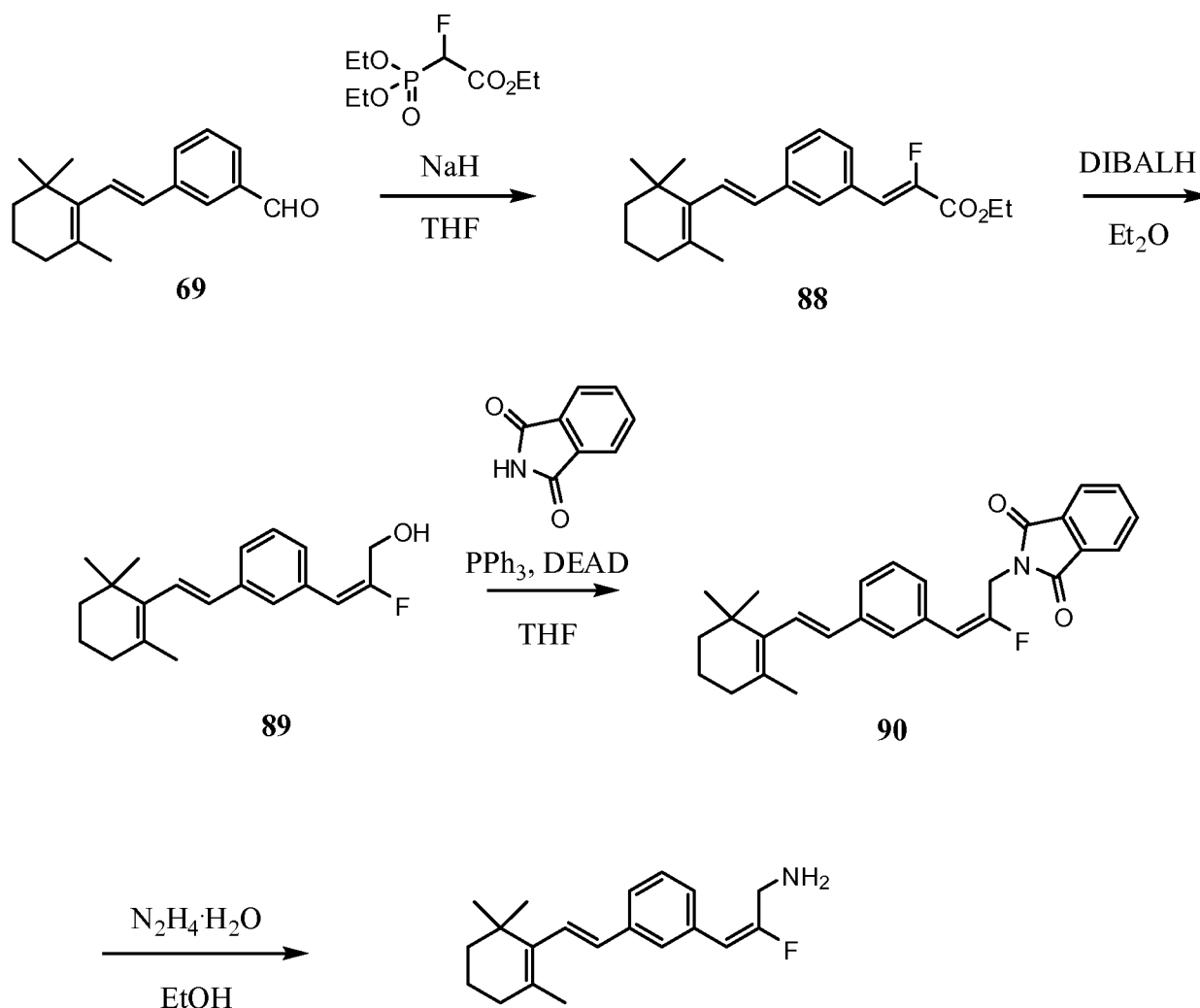
SCHEME 30
