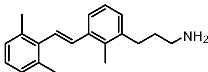
SCHEME 13
