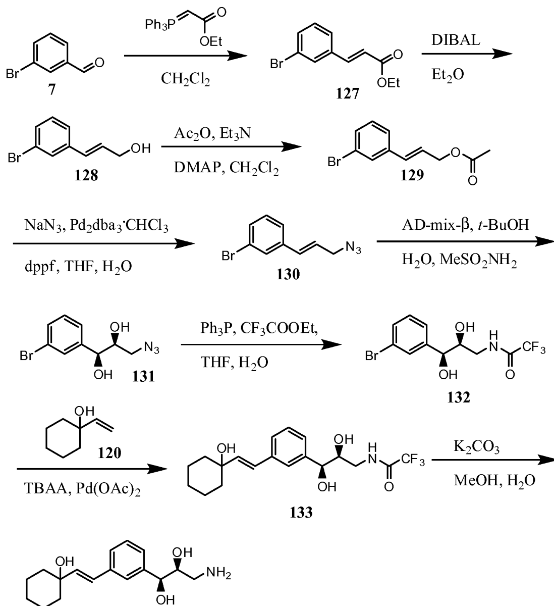
SCHEME 43
