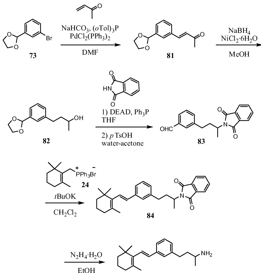
SCHEME 28
