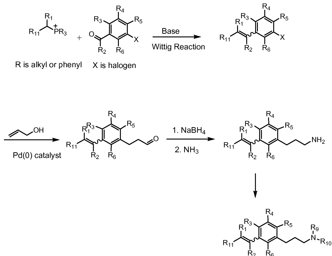
SCHEME I
