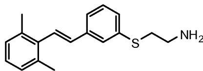
SCHEME 5
