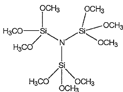
Nonamethoxytrisilazoxane (NMTS)
