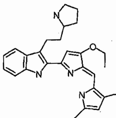
Compound 24
