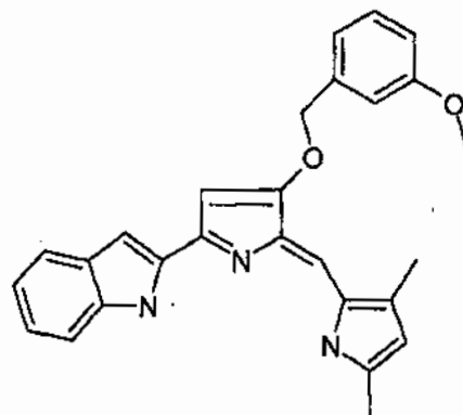
Compound 51
