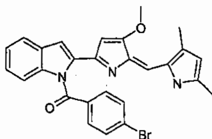
Compound 55
