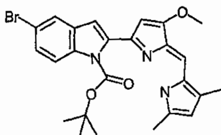
Compound 21
