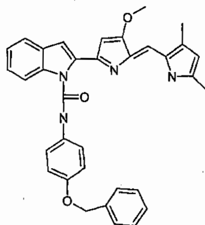
Compound 54
