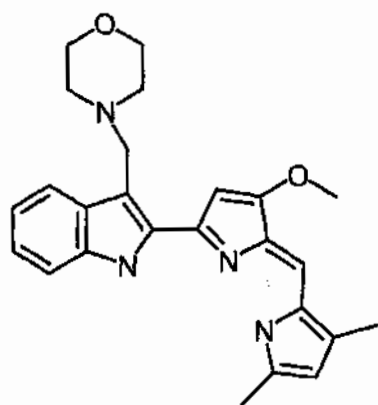
Compound 6 2-[5-(3,5-Dimethyl-1H-pyrrol-2-ylmethylene)-4-methoxy-5H-pyrrol-2-yl]-3-morpholin-4-ylmethyl-1H-indole;
