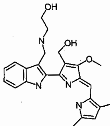
Compound 9 2-((2-[5-(3,5-Dimethyl-1H-pyrrol-2-ylmethylene)-3-hydroxymethyl-4-methoxy-5H-pyrrol-2-yl]-1H-indol-3-ylmethyl)-amino)ethanol;
