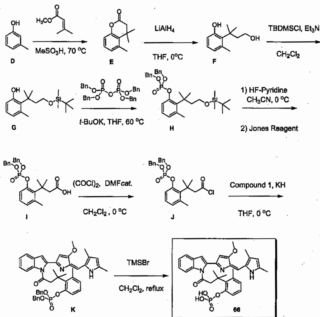
Scheme 3
