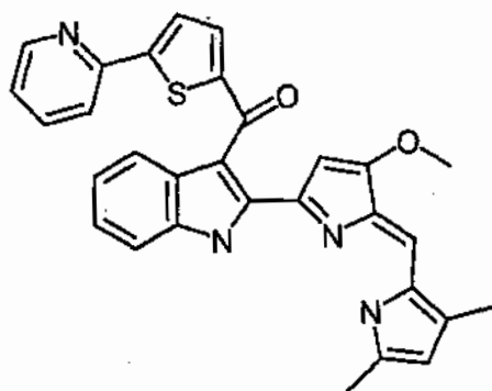
Compound 22
