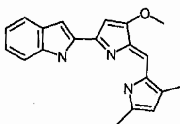
Compound 1
