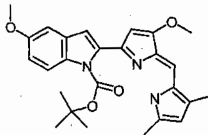
Compound 30
