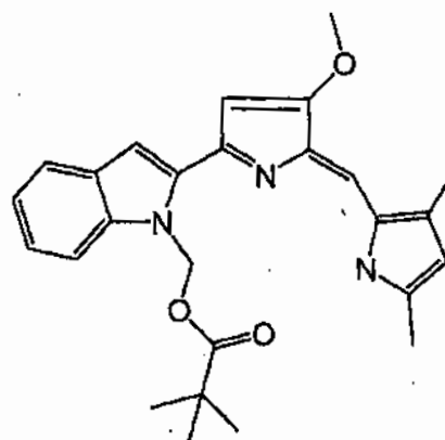
Compound 64
