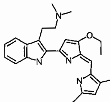
Compound 31
