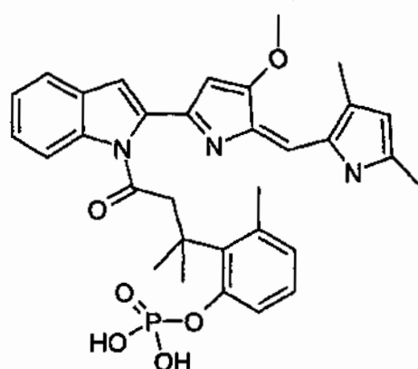
Compound 66
