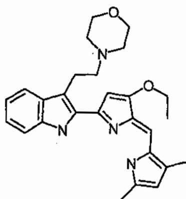
Compound 14
