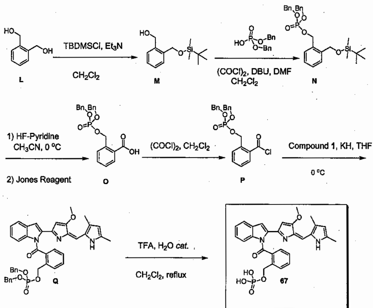
Scheme 4
