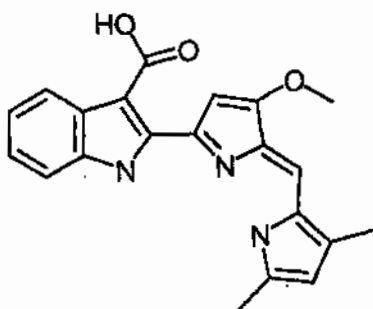
Compound 16
