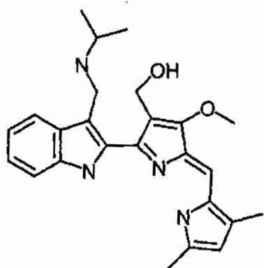
Compound 11
