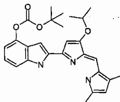
Compound 38
