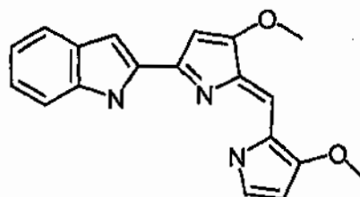
Compound 3 2-[4-Methoxy-5-(3-methoxy-1H-pyrrol-2-ylmethylene)-5H-pyrrol-2-yl]-1H-indole;
