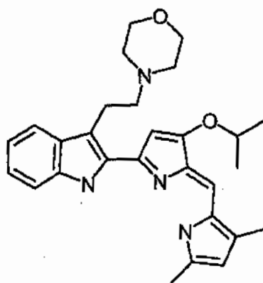
Compound 32
