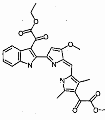
Compound 20
