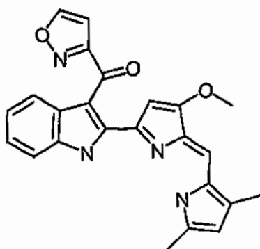
Compound 23
