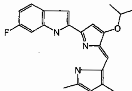
Compound 45
