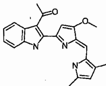
Compound 25
