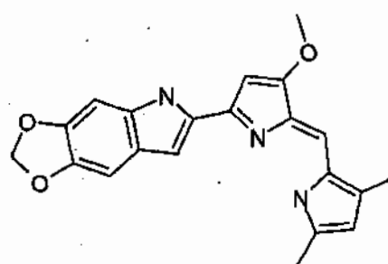
Compound 60
