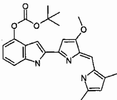
Compound 36
