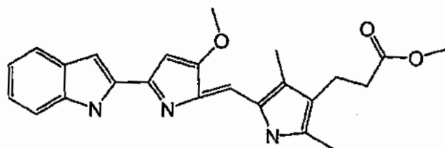
Compound 63
