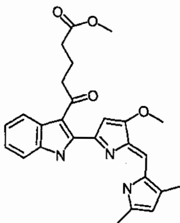
Compound 19
