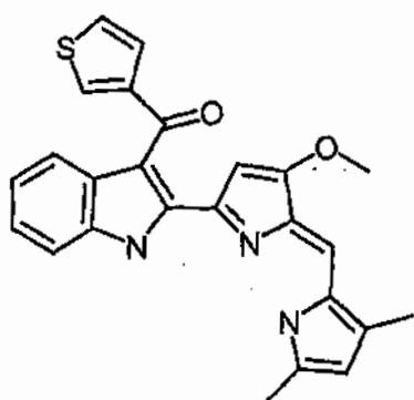
Compound 12
