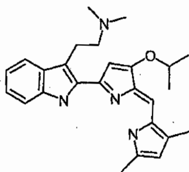
Compound 33
