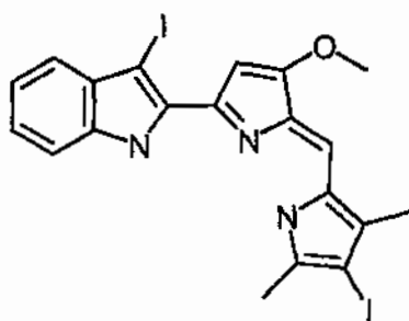
Compound 17
