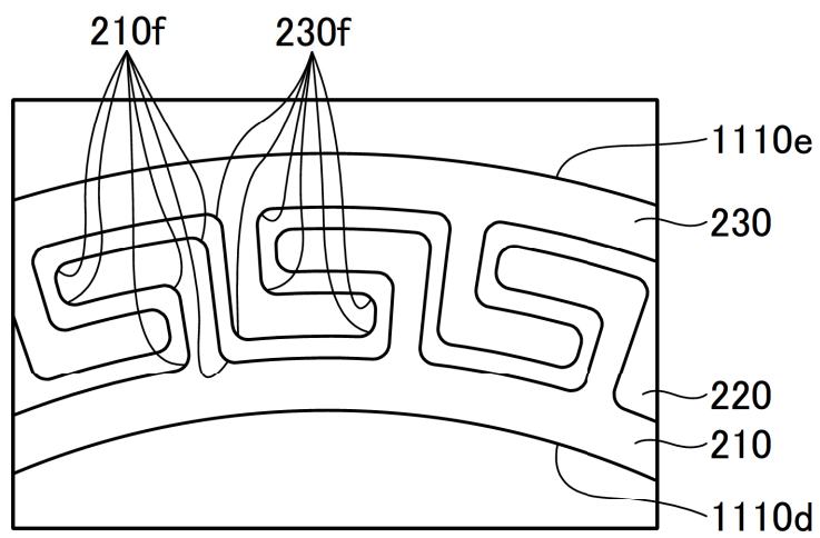
FIG.7D
