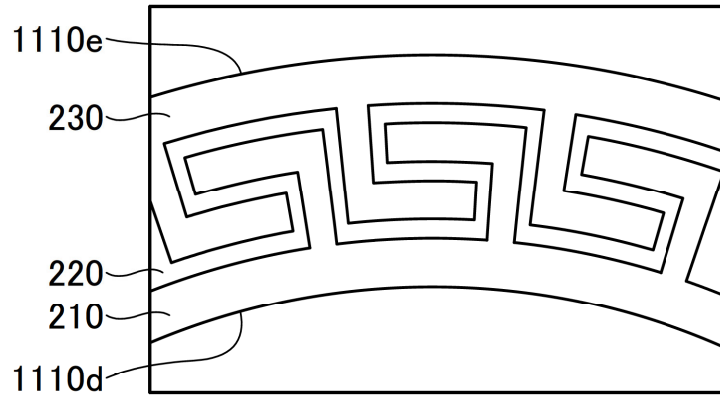
7/13 FIG.7C
