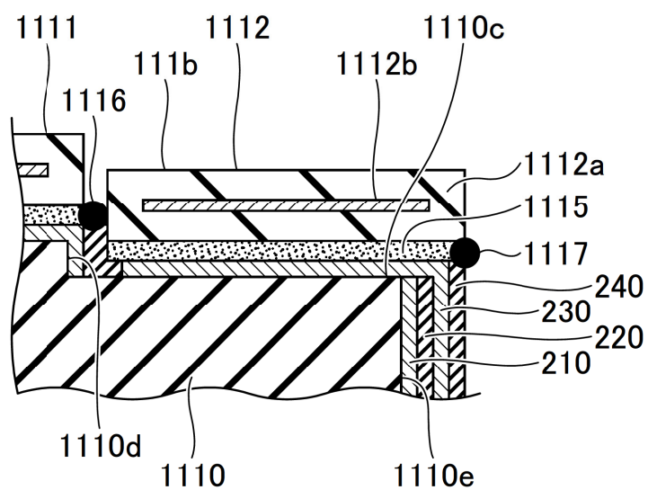
6/13 FIG.6
