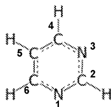
Pyrimidine
