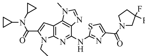
N,N -dicyclopropyl-4-(4-(3,3-difluoropyrrolidine-1-carbonyl)thiazol-2-ylamino)-6-ethyl-1-methyl-1,6-dihydroimidazo[4,5-d]pyrrolo[2,3-b]pyridine-7-carboxamide
