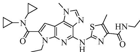
15 2-(7-(dicyclopropylcarbamoyl)-6-ethyl-1-methyl-1,6-dihydroimidazo[4,5-d]pyrrolo[2,3-b]pyridine-4-ylamino)-N-ethyl-5-methylthiazole-4-carboxamide
