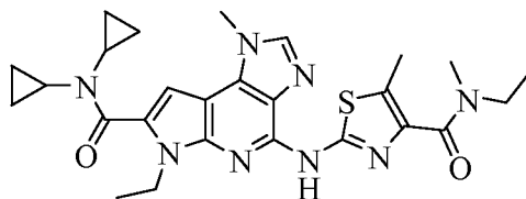
2-(7-(dicyclopropylcarbamoyl)-6-ethyl-1-methyl-1,6-dihydroimidazo[4,5-d]pyrrolo[2,3-b]pyridin-4-ylamino)-N-ethyl-N,5-dimethylthiazole-4-carboxamide
