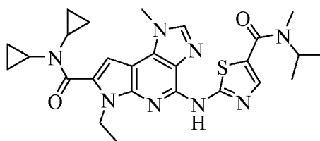
2-(7-(dicyclopropylcarbamoyl)-6-ethyl-1-methyl-1,6-dihydroimidazo[4,5-d]pyrrolo[2,3-b]pyridin-4-ylamino)-N-isopropyl-N-methylthiazole-5-carboxamide
