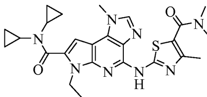
2-(7-(dicyclopropylcarbamoyl)-6-ethyl-1-methyl-1,6-dihydroimidazo[4,5-d]pyrrolo[2,3-b]pyridin-4-ylamino)-N,N,4-trimethylthiazole-5-carboxamid
