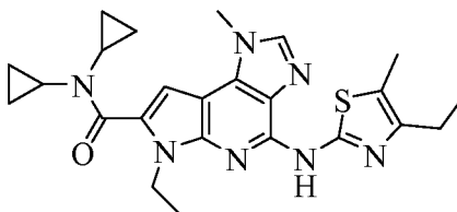
N,N -dicyclopropyl-6-ethyl-4-(4-ethyl-5-methylthiazol-2-ylamino)-1-methyl-1,6-dihydroimidazo[4,5-d]pyrrolo[2,3-b]pyridine-7-carboxamide
