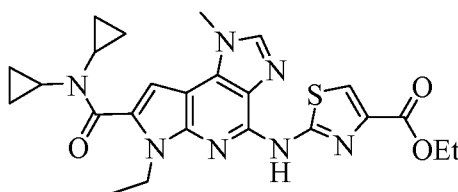
Ethyl 2-(7-(dicyclopropylcarbamoyl)-6-ethyl-1-methyl-1,6-dihydroimidazo[4,5-d]pyrrolo[2,3-b]pyridin-4-ylamino)thiazole-4-carboxylate
