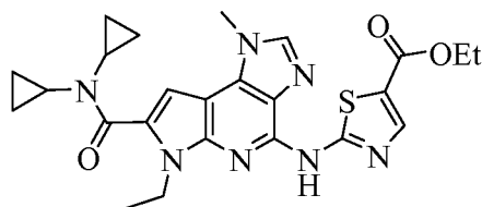
Ethyl 2-(7-(dicyclopropylcarbamoyl)-6-ethyl-1-methyl-1,6-dihydroimidazo[4,5-d]pyrrolo[2,3-b]pyridin-4-ylamino)thiazole-5-carboxylate
