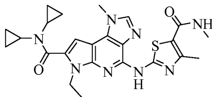
2-(7-(dicyclopropylcarbamoyl)-6-ethyl-1-methyl-1,6-dihydroimidazo[4,5-d]pyrrolo[2,3-b]pyridin-4-ylamino)-N,4-dimethylthiazole-5-carboxamide
