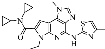
N,N -dicyclopropyl-6-ethyl-1-methyl-4-(4-methylthiazol-2-ylamino)-1,6-dihydroimidazo[4,5-d]pyrrolo[2,3-b]pyridine-7-carboxamide
