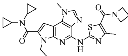
4-(5-(azetidine-1-carbonyl)-4-methylthiazol-2-ylamino)-N,N-dicyclopropyl-6-ethyl-1-methyl-1,6-dihydroimidazo[4,5-d]pyrrolo[2,3-b]pyridine-7-carboxamide
