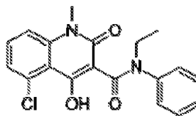
Laquinimod
