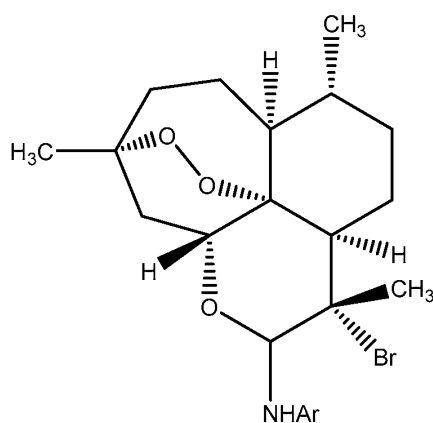
(Formula I-M'),
