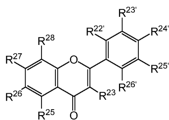
(Formula II-A),
