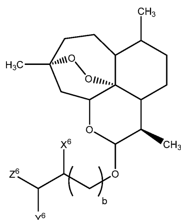
(Formula I-F),
