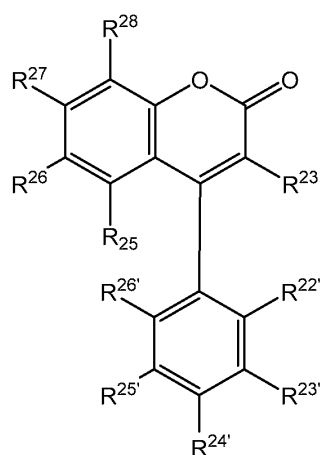
(Formula II-C),
