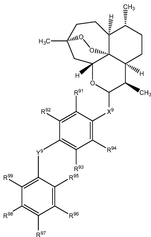
(Formula I-I).
