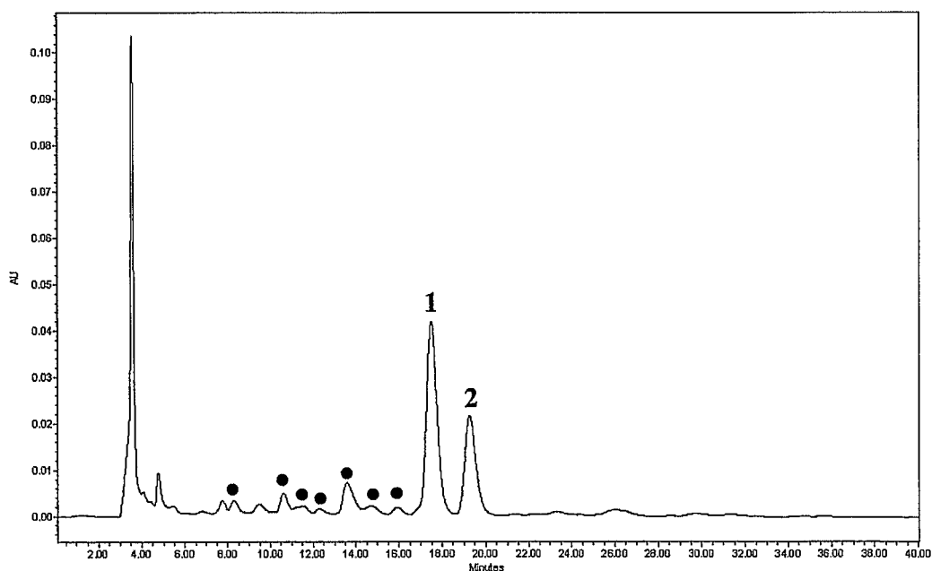
Figure 3: LC-PDA (275 nm) of decolourised caramel. Denoted peaks: Compound 1: 2,6-deoxyfructosazine and 2: 2,5-deoxyfructosazine.
