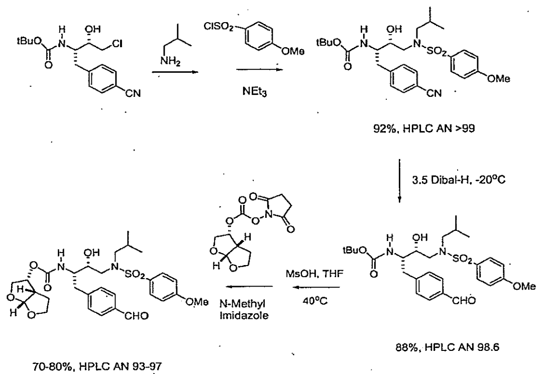
Scheme 4.
