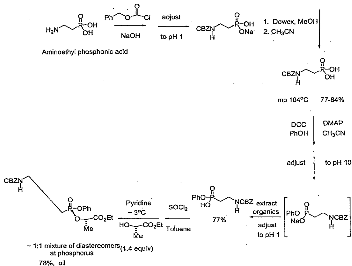
Scheme 5.
