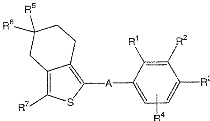
Formula (I)
