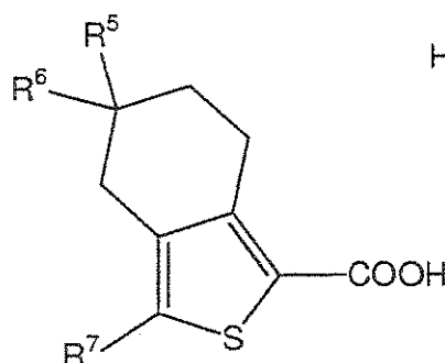
Structure 1
