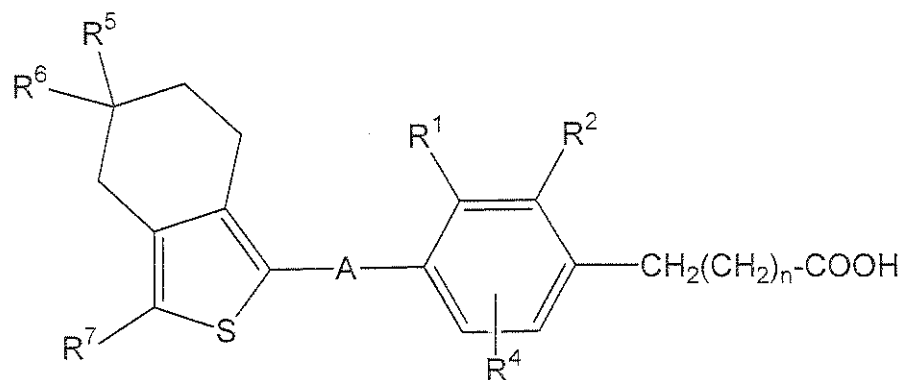
Formula (III)
