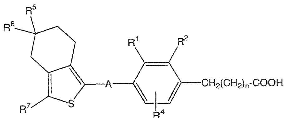
Formula (III)
