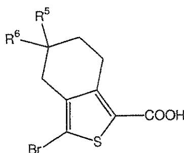
Structure 18
