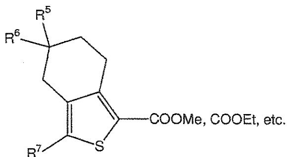
Structure 13
