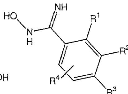
Structure 11
