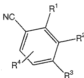
Structure 12
