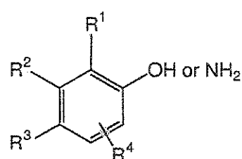
Structure 9
