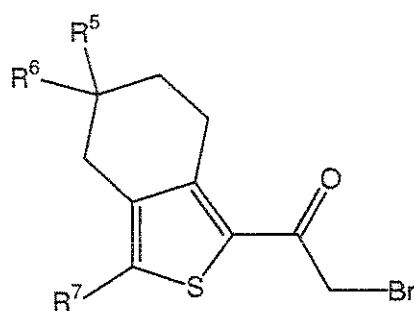
Structure 8
