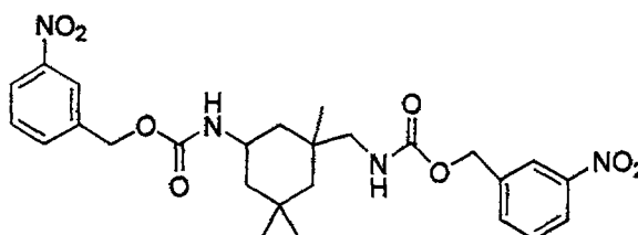
"Bis( m -nitrobenzyl carbamate) of IPDI"
