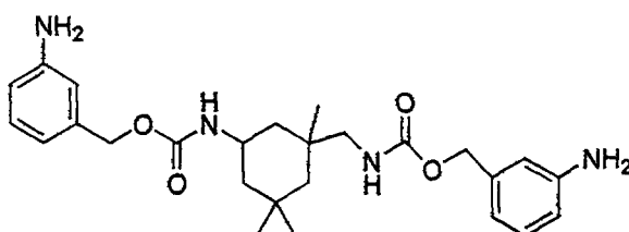
"Bis( m -aminobenzyl carbamate) of IPDI"
