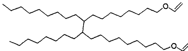
"Dimer Divinyl Ether" (and cyclic isomers)
