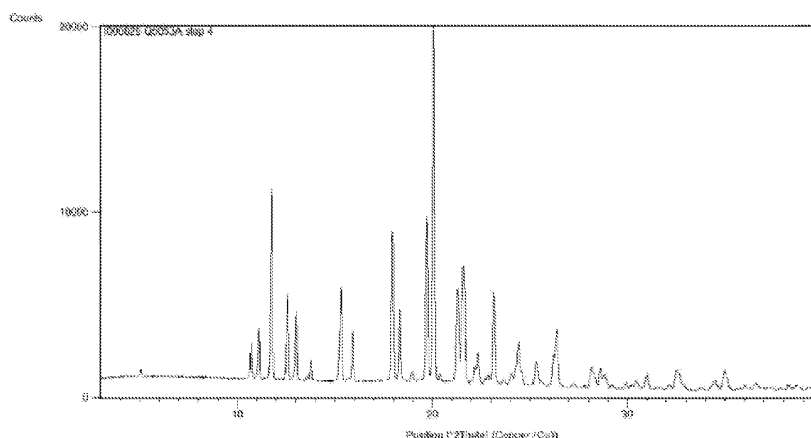
FIG. 1 XRPD of Formula II Monohydrate
