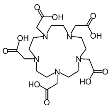
PEPA
