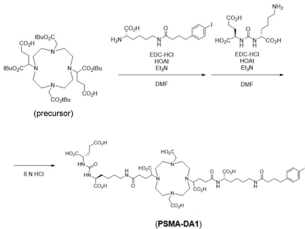
Scheme (V-1)
