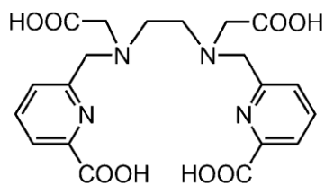
H 4 octapa
