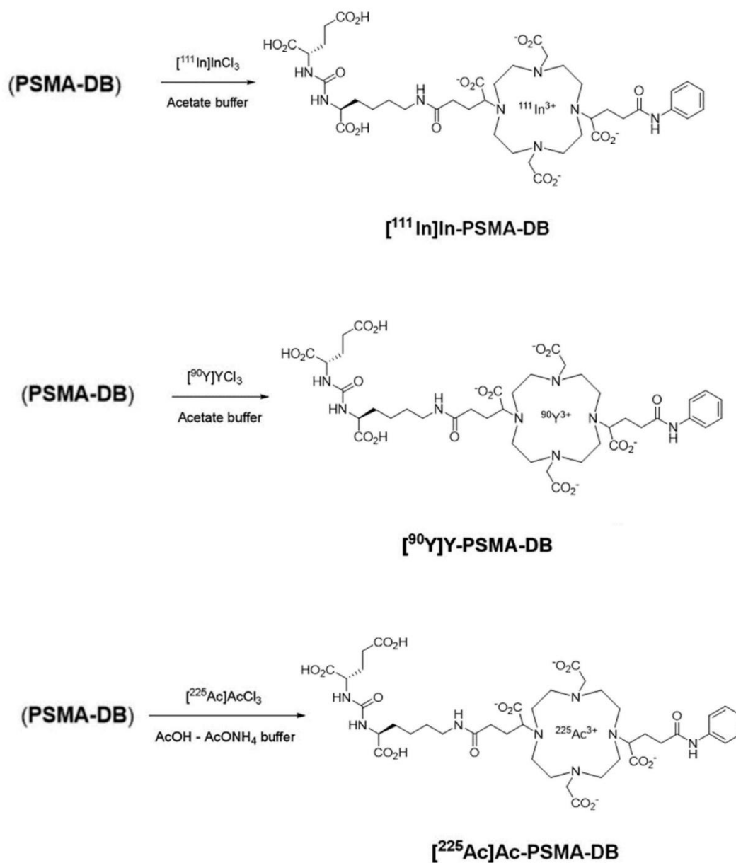
Scheme (VI-2)
