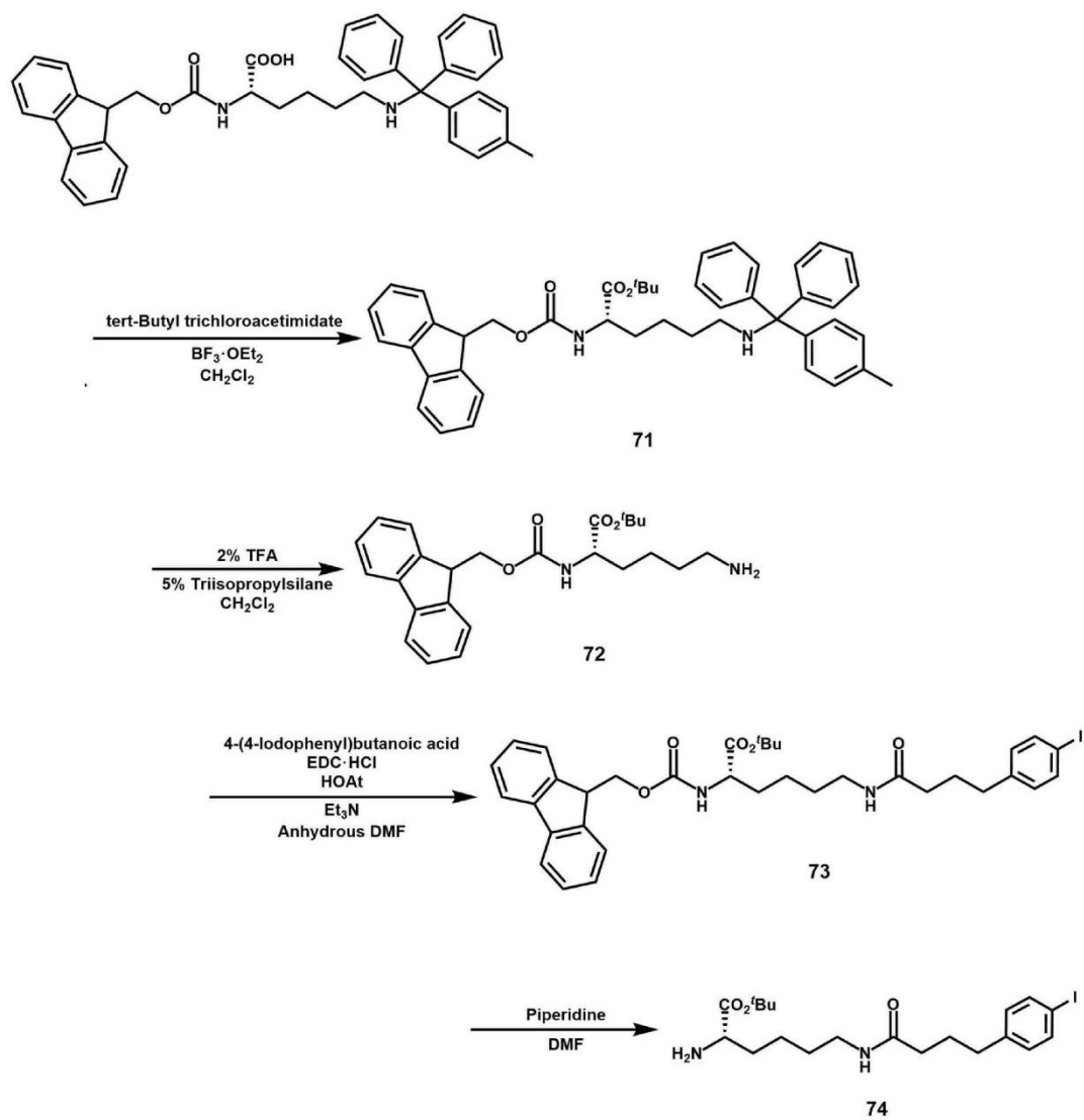
Scheme (VIII-1)
