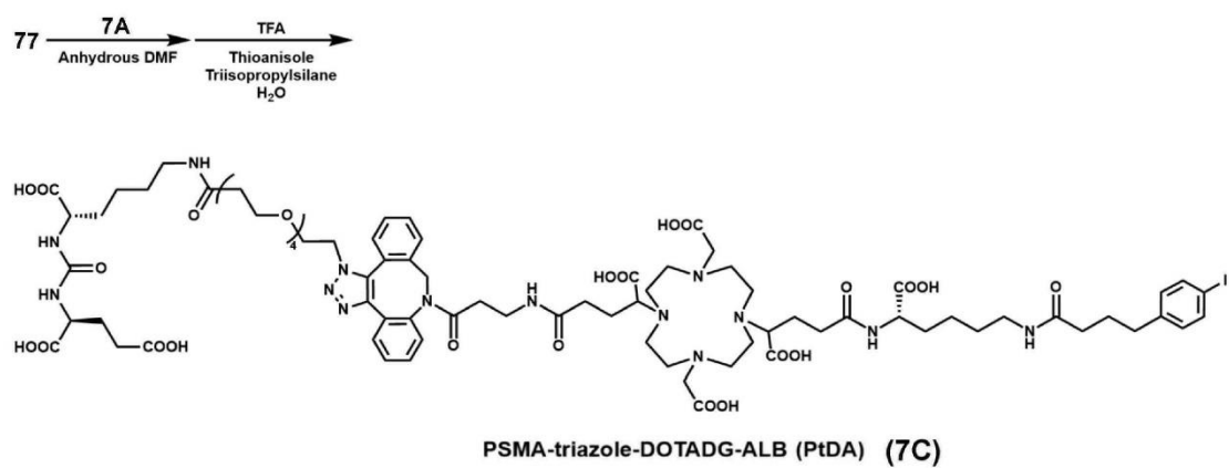
Scheme (VIII-3)
