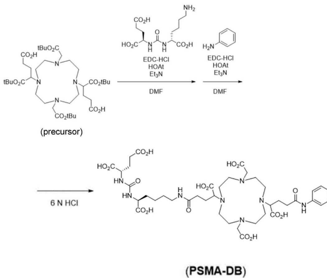
Scheme (VI-1)
