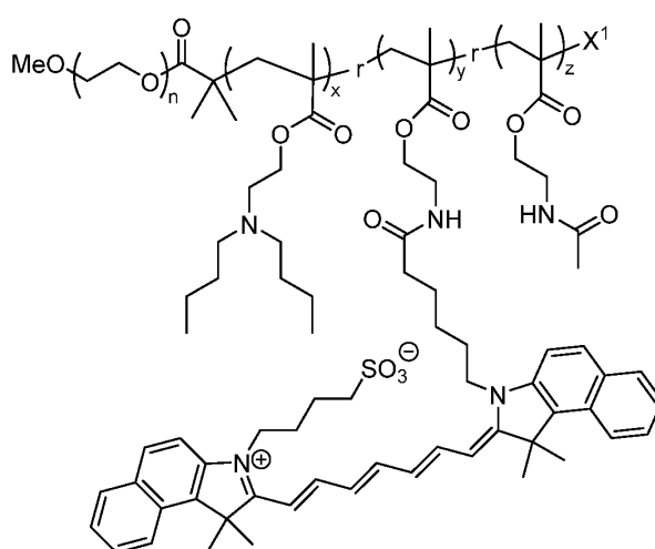
Formula (II),
