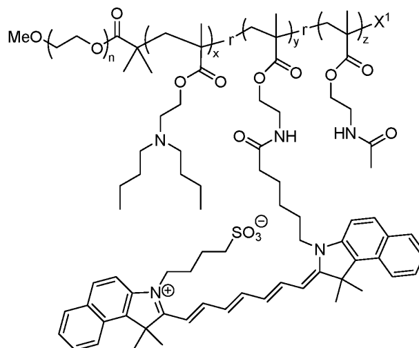
Formula (II),
