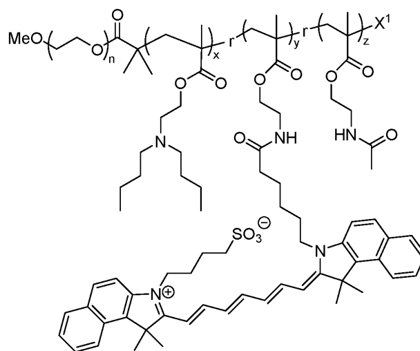
Formula (II),
