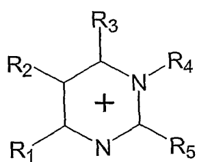
Pyrimidinium
