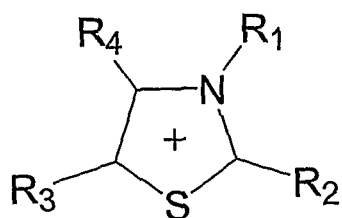
Thiazolium
