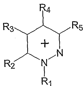
Pyridazinium
