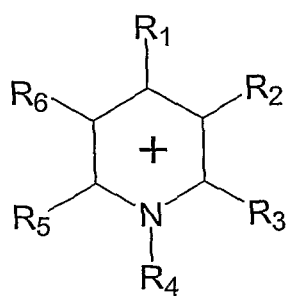
Pyridinium
