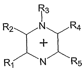
Pyrazinium
