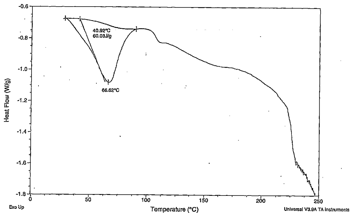
Fig. 2b DSC of Polymorph II
