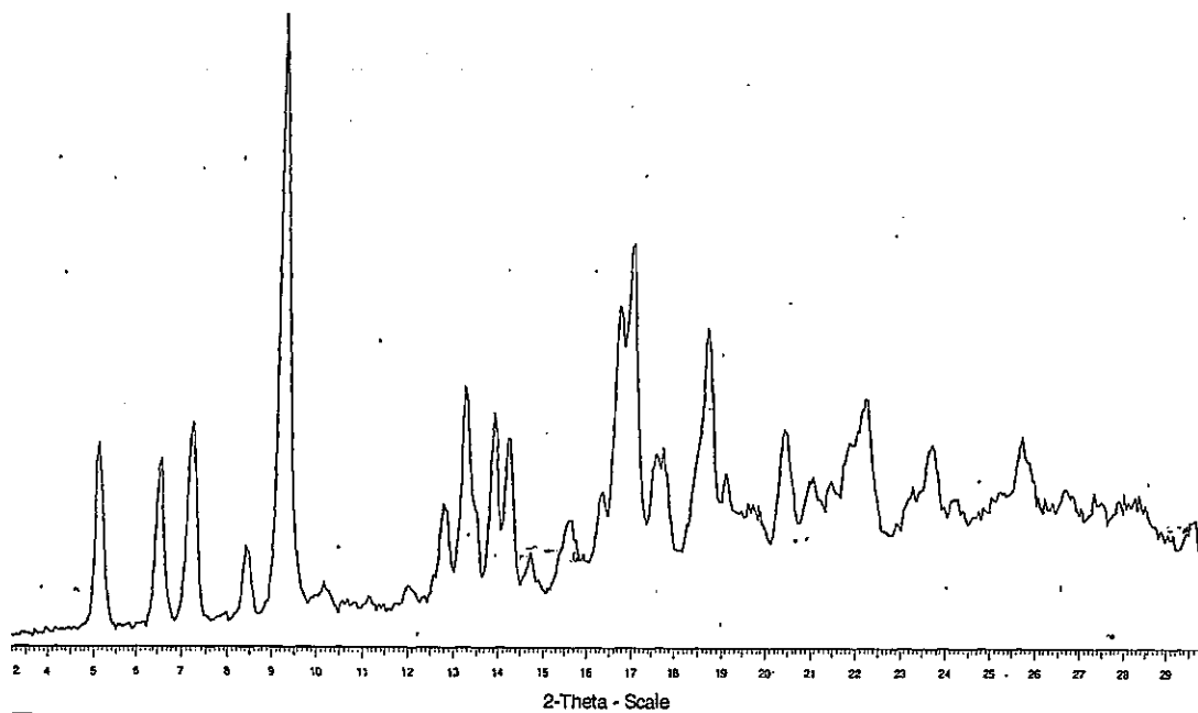
Fig. 1d XRPD of Polymorph IV
