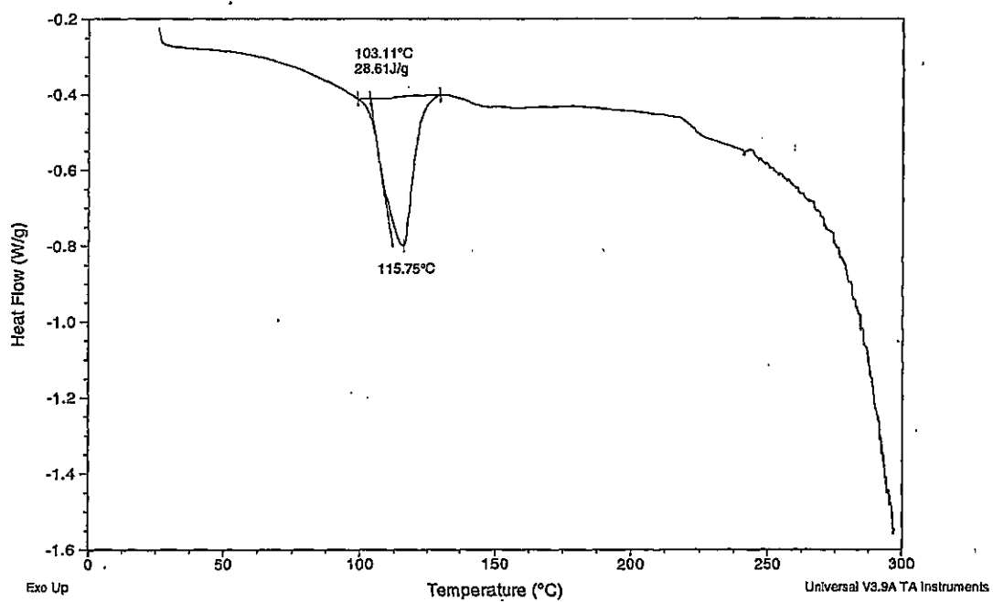
Fig. 2f DSC of Polymorph VII
