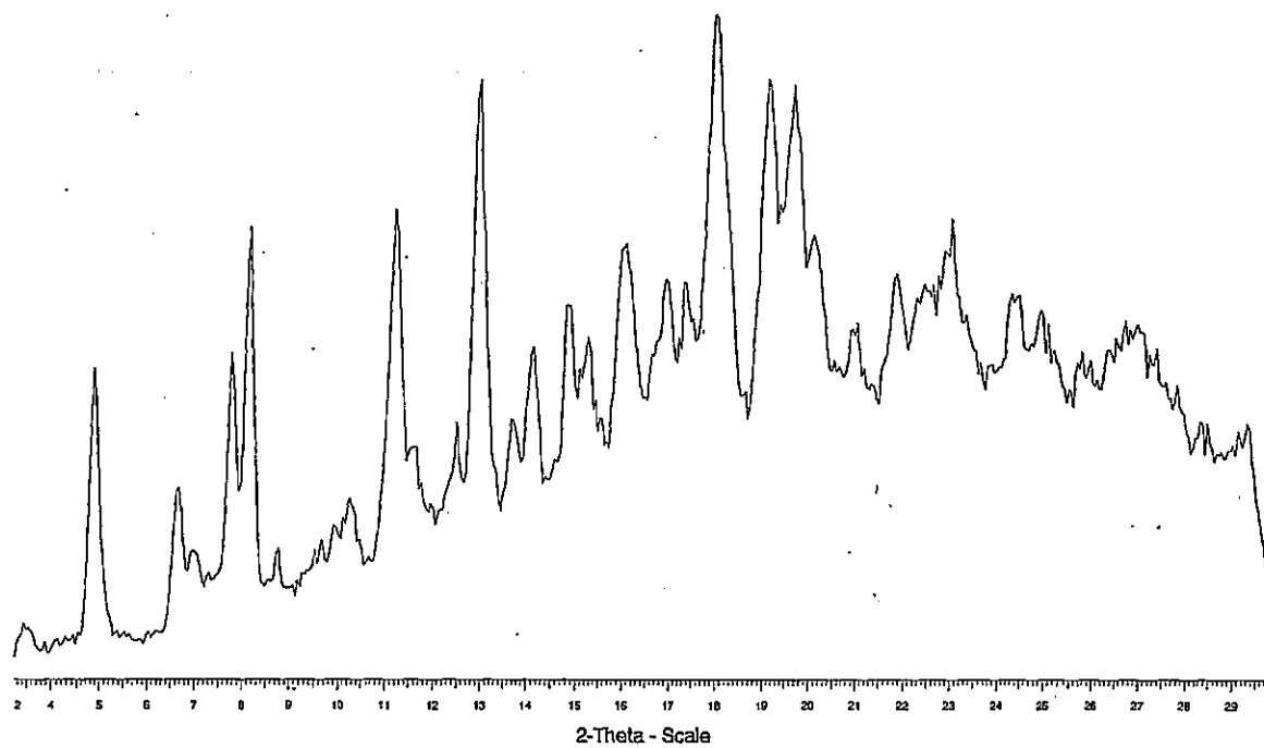
Fig. 1g XRPD of Polymorph VII
