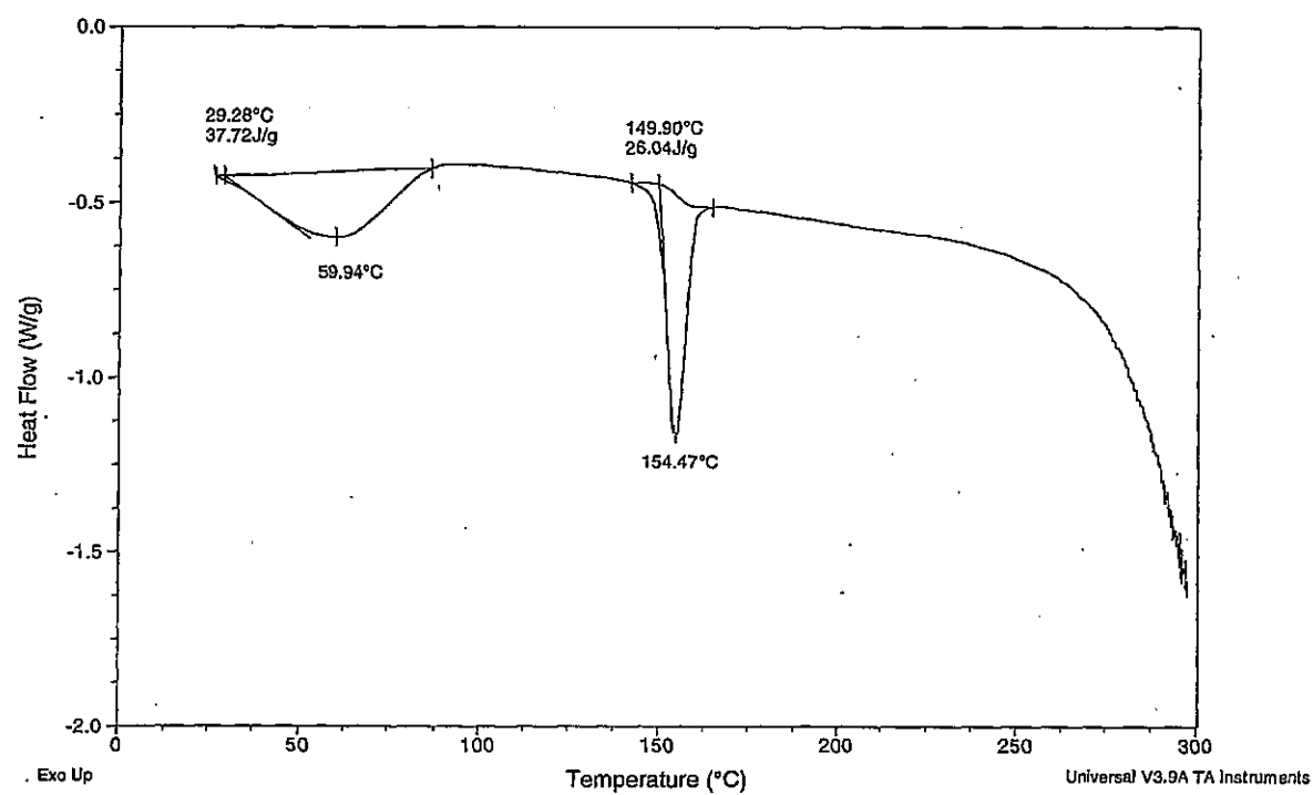
Fig. 2d DSC of Polymorph V
