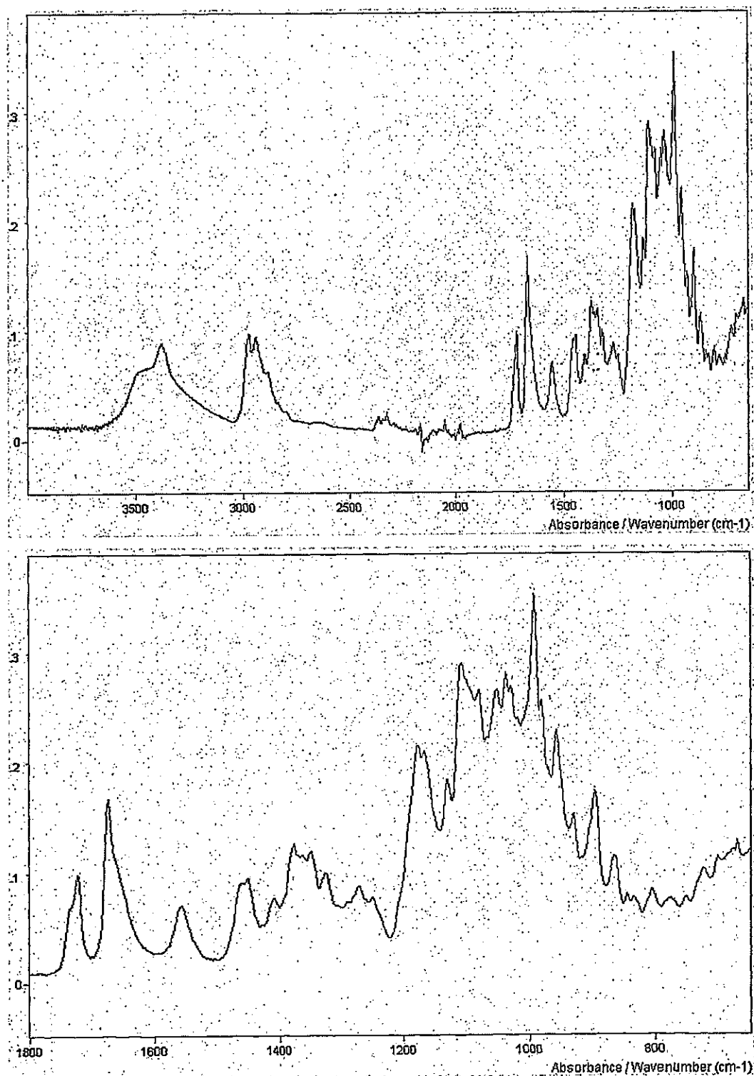
Fig.5 FT-IR spectrum for Polymorph IV
