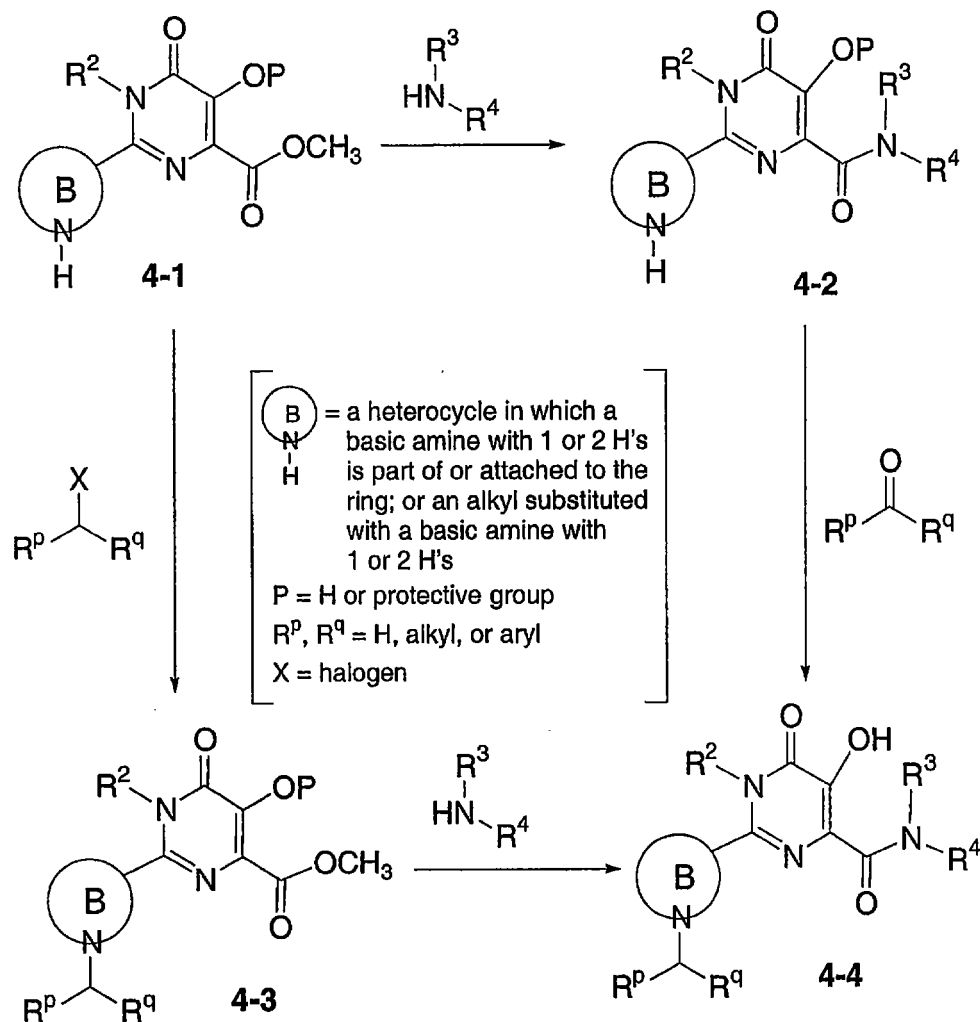
Scheme 4
