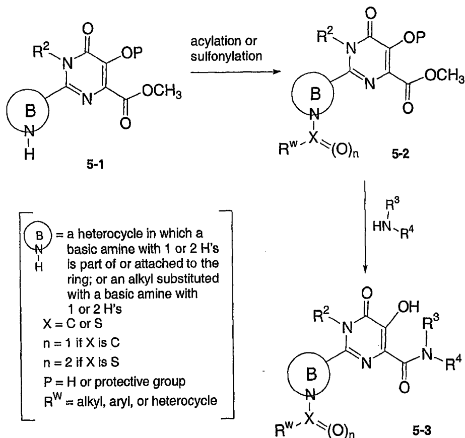
Scheme 5
