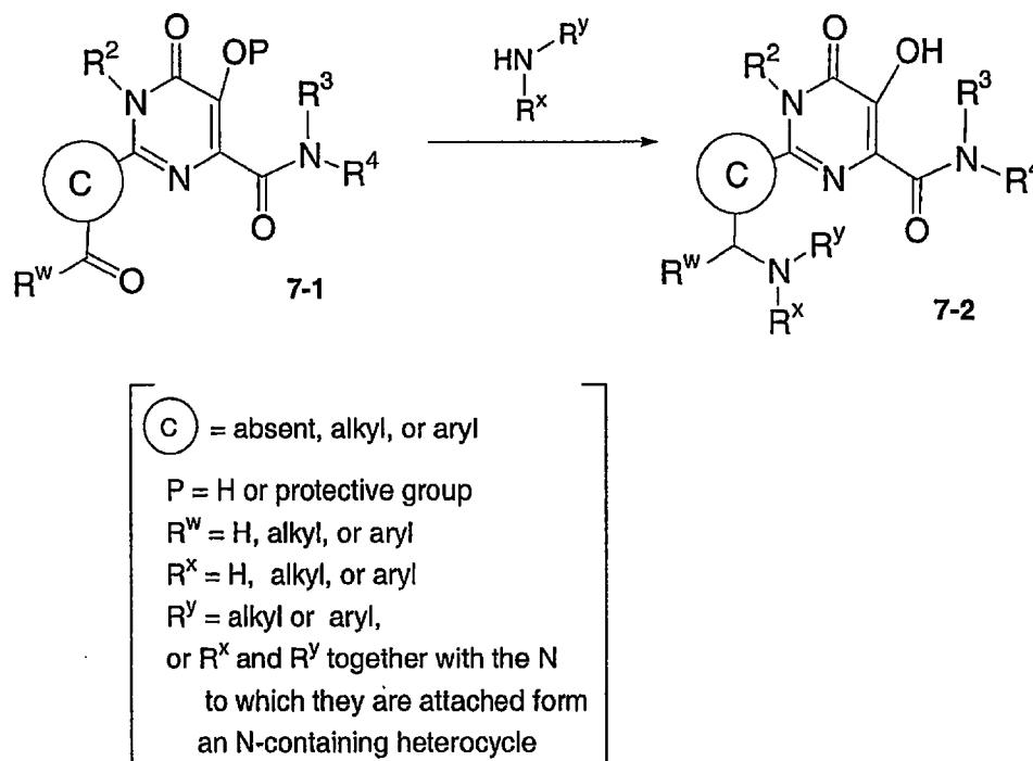
Scheme 7
