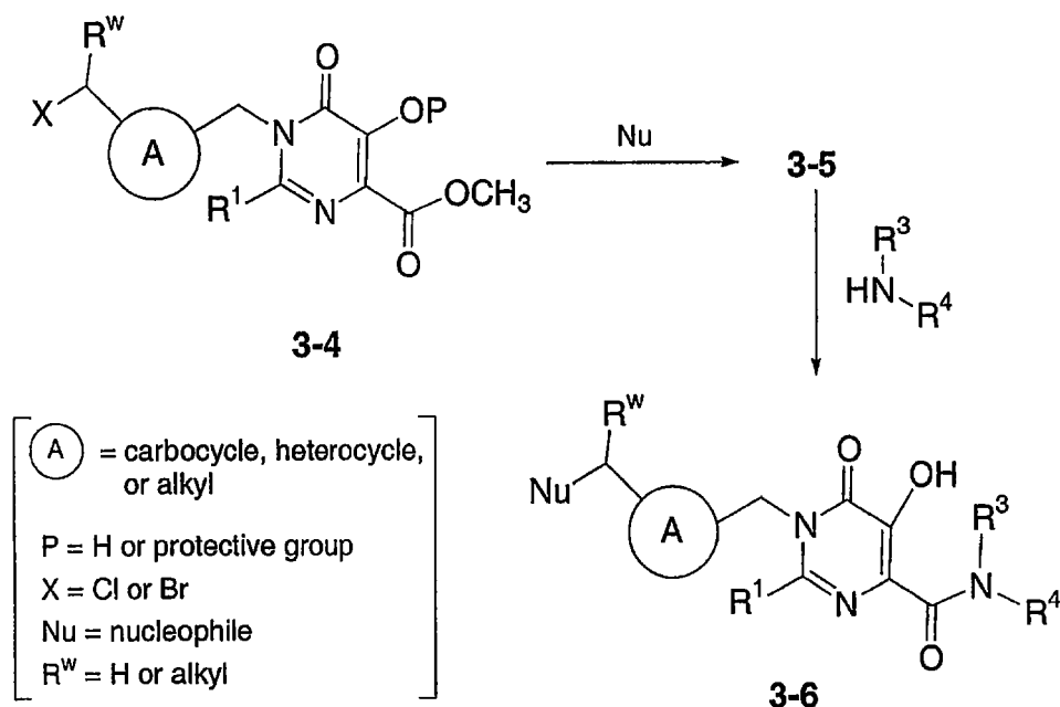
Scheme 3 - Part 2
