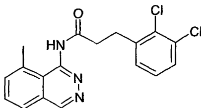
3-(2,3-dichlorophenyl)-N-(8-methyl-phthalazin-1-yl)-propionamide ("A26")
