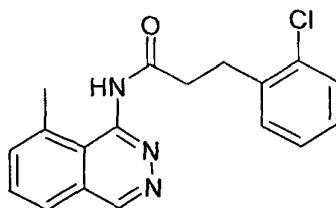
3-(2-chlorophenyl)-N-(8-methyl-phthalazin-1-yl)-propionamide ("A25")
