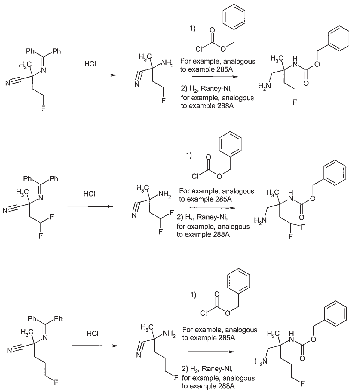
Scheme 11:
