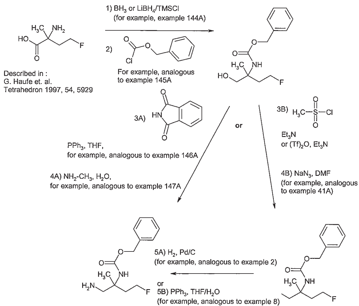
Scheme 8:
