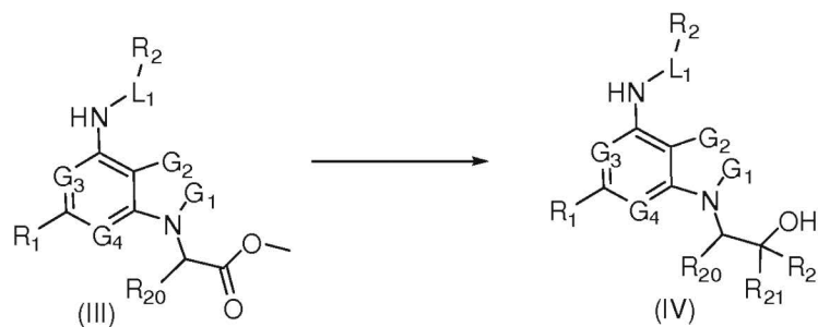
Reaction Scheme 5
