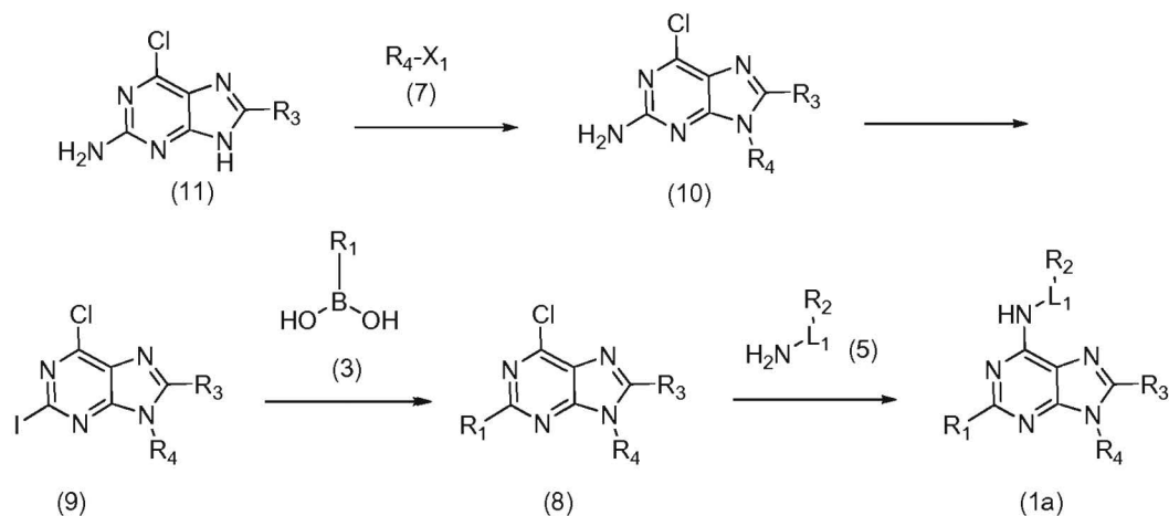
Reaction Scheme 2
