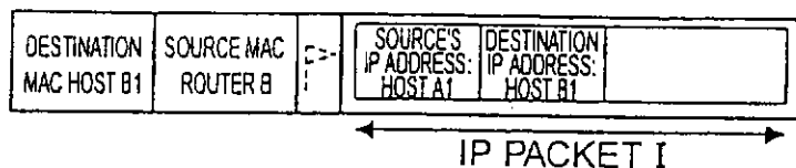
ETHERNET FRAME VII
