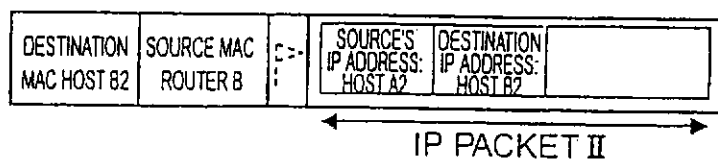
ETHERNET FRAME VII
