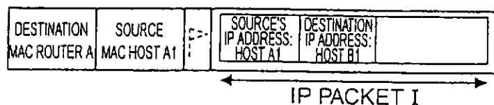
ETHERNET FRAME II
