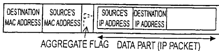
ETHERNET FRAME I
