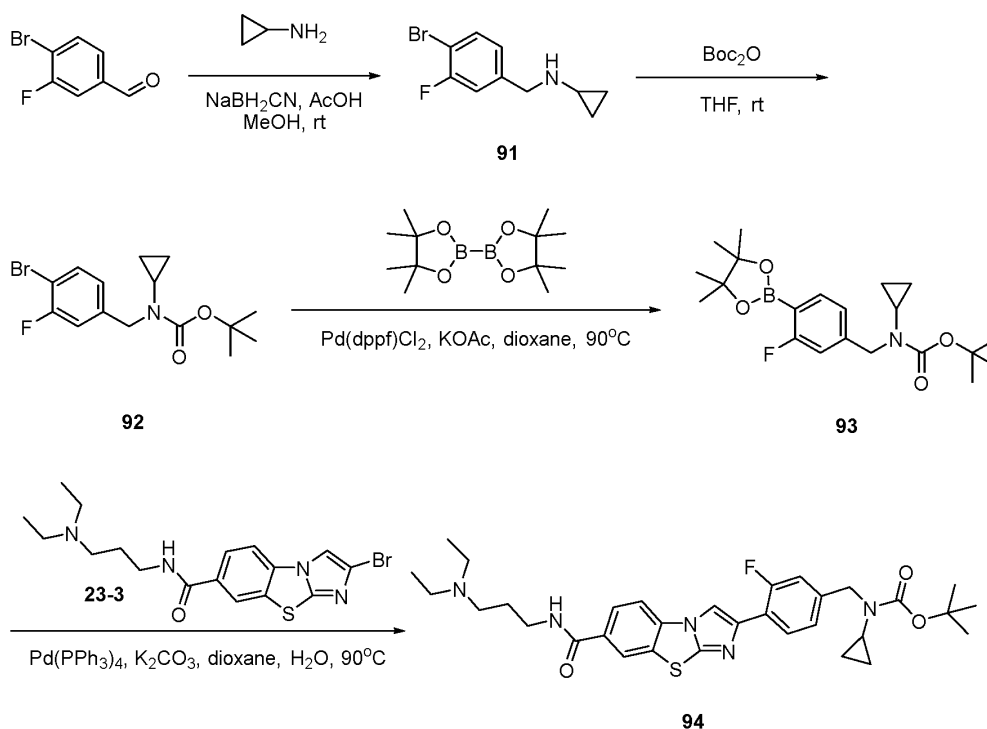
Scheme 48
