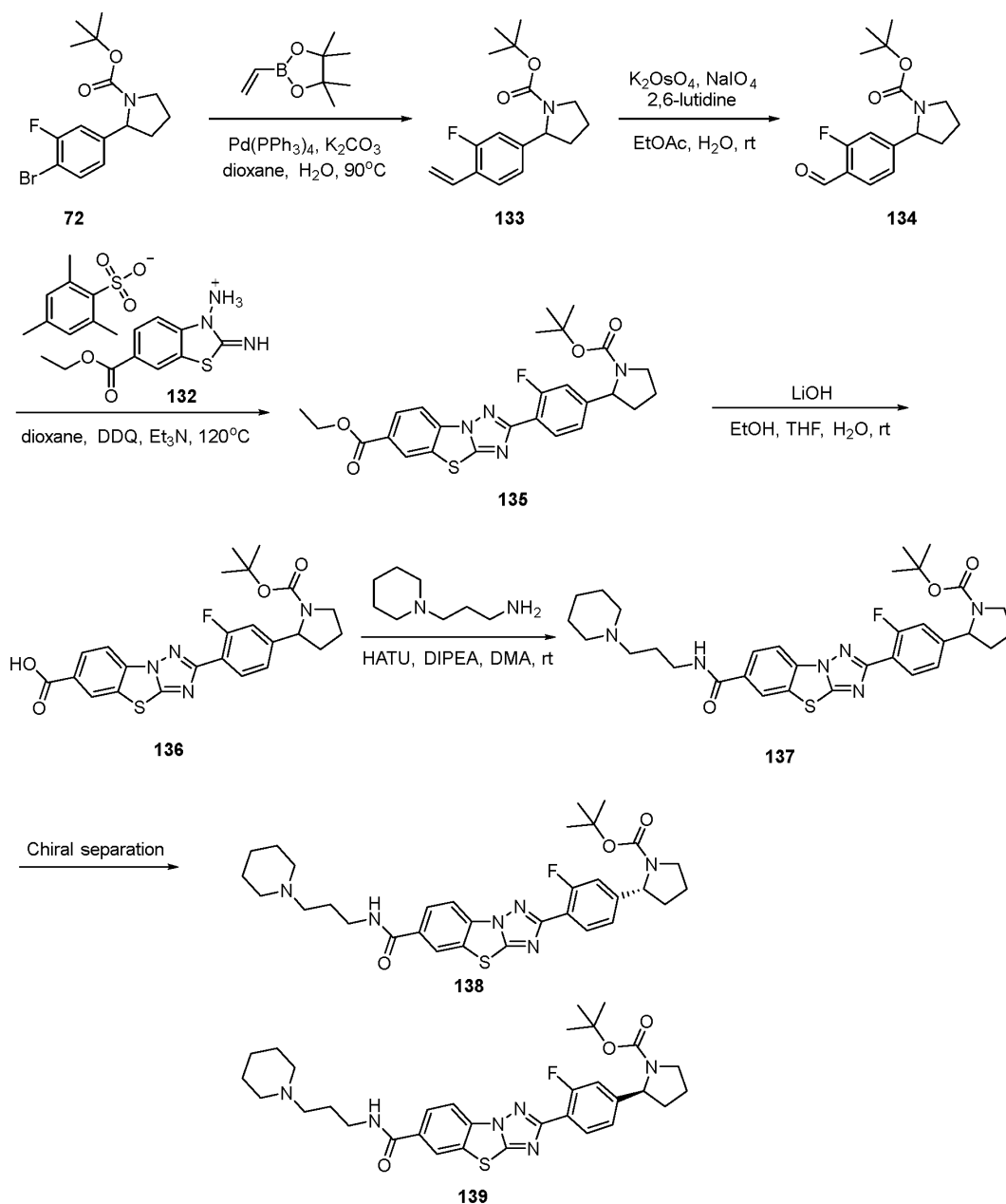
Scheme 59
