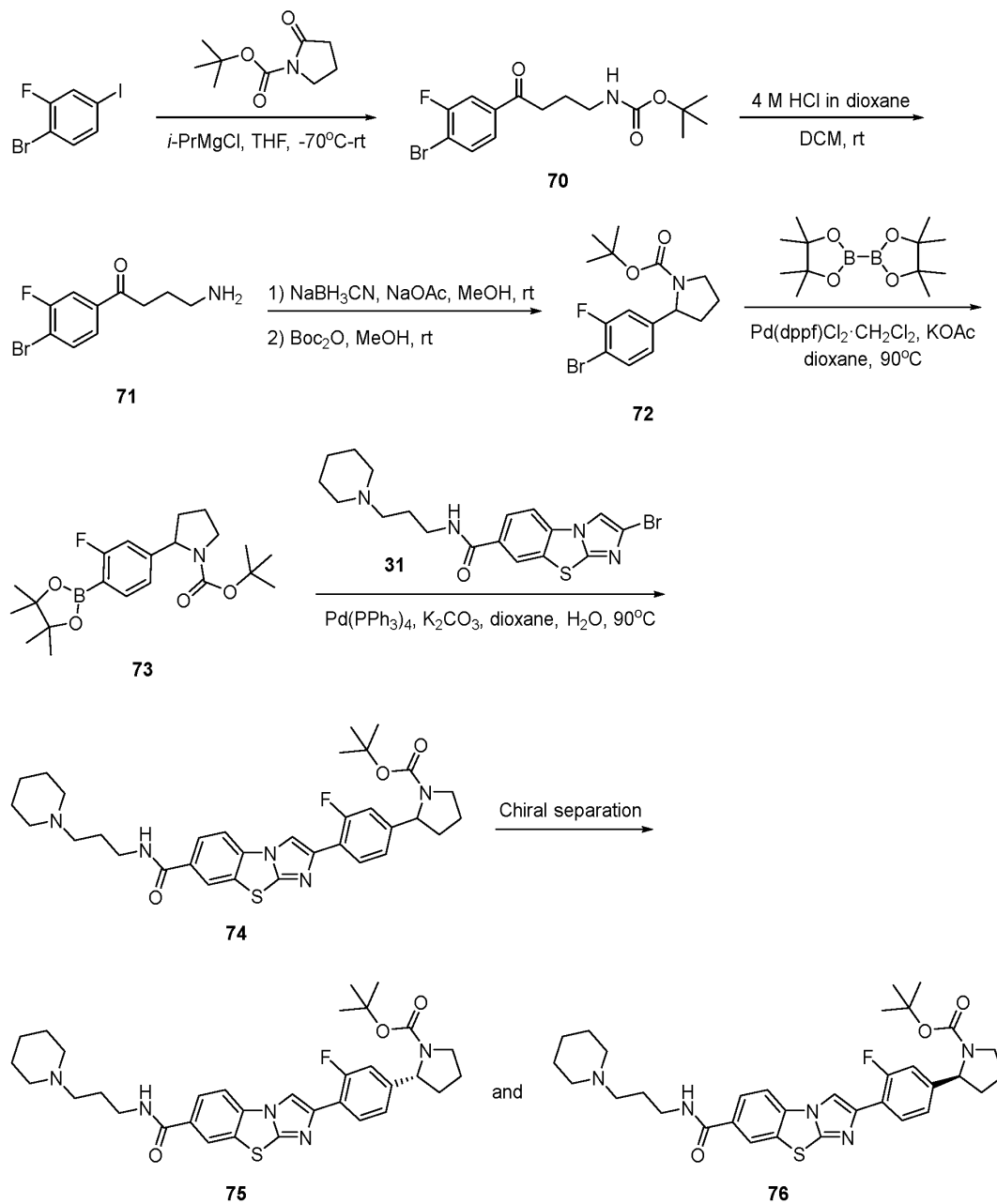
Scheme 44
