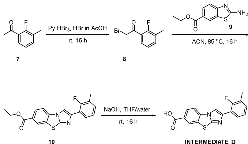
Scheme 26
