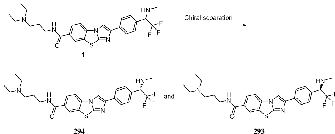
Scheme 75
