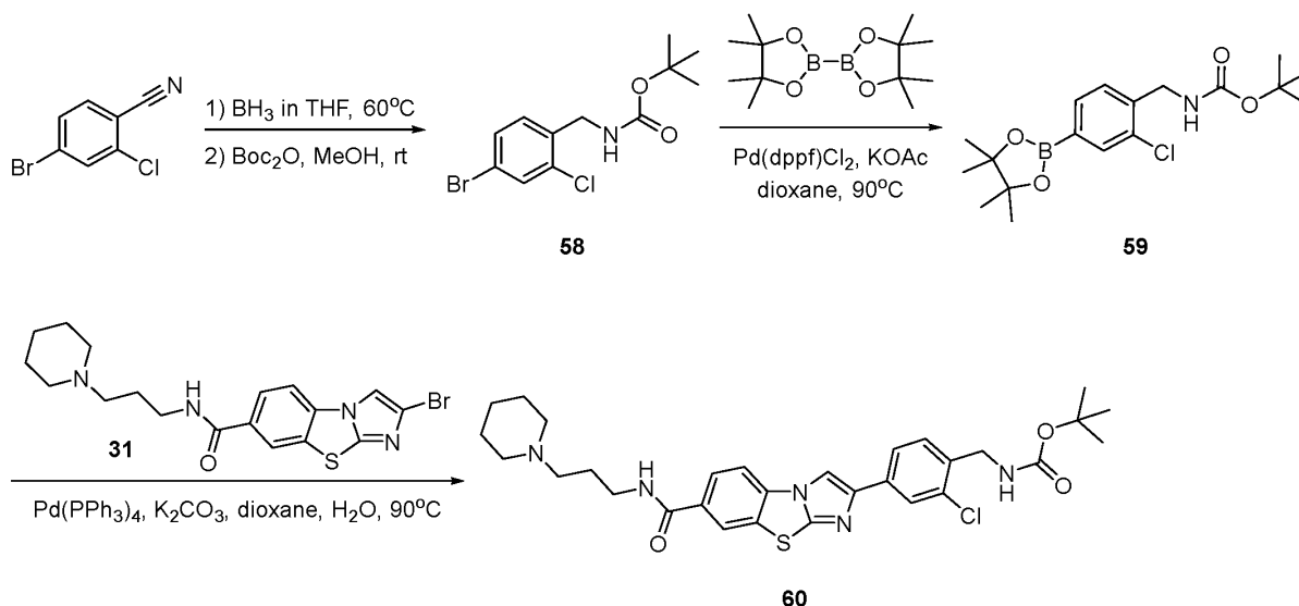
Scheme 40
