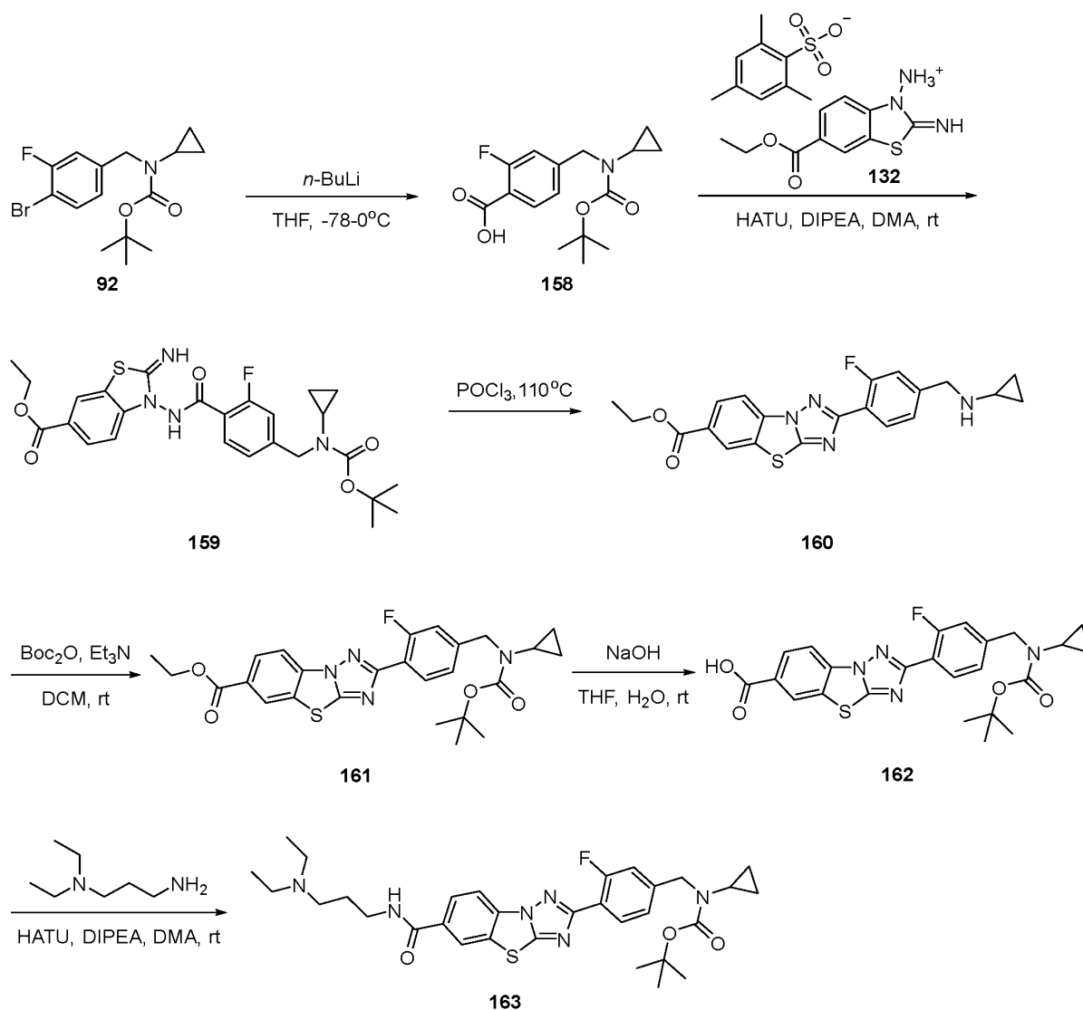
Scheme 63
