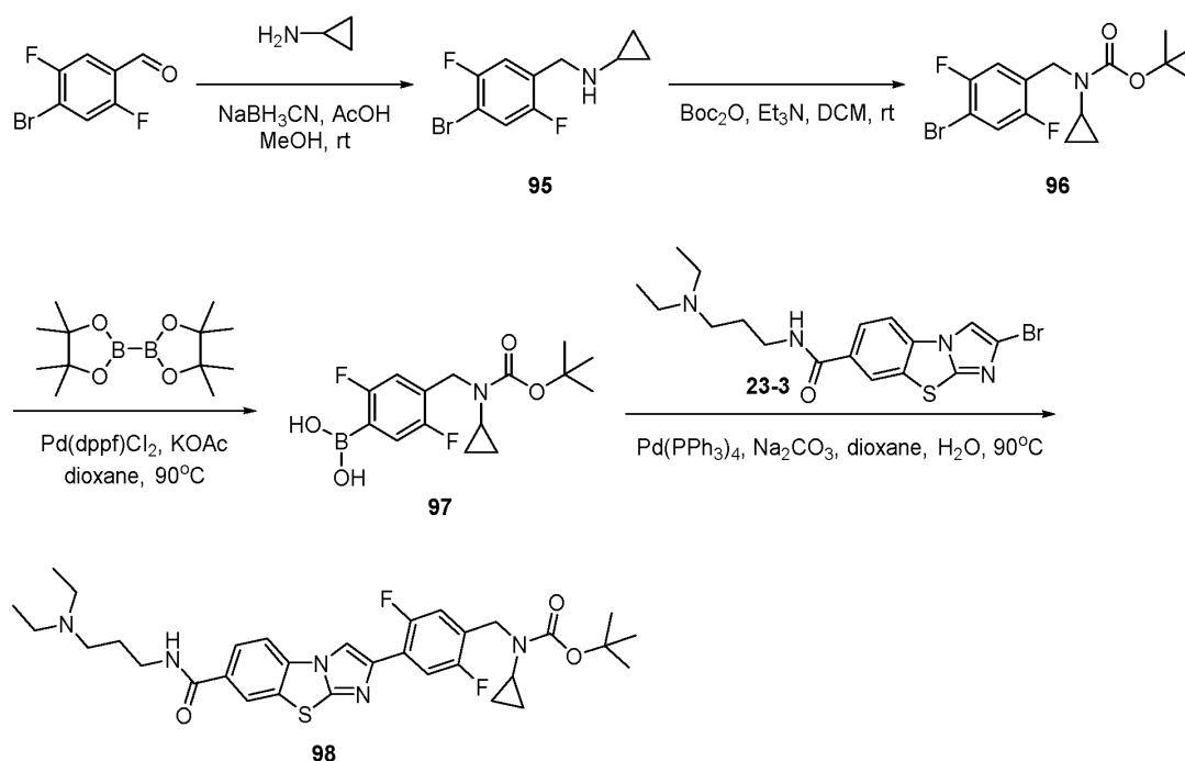
Scheme 49
