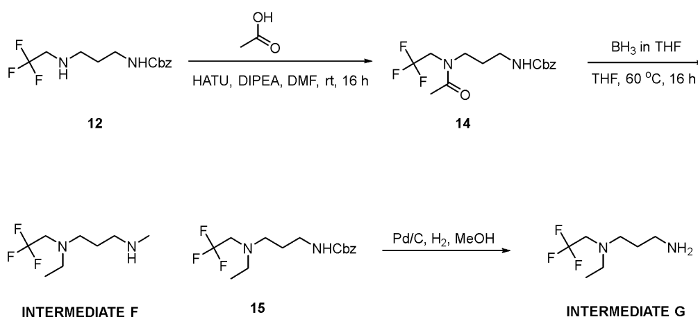
Scheme 28
