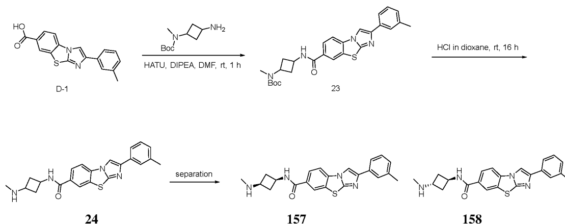
Scheme 67
