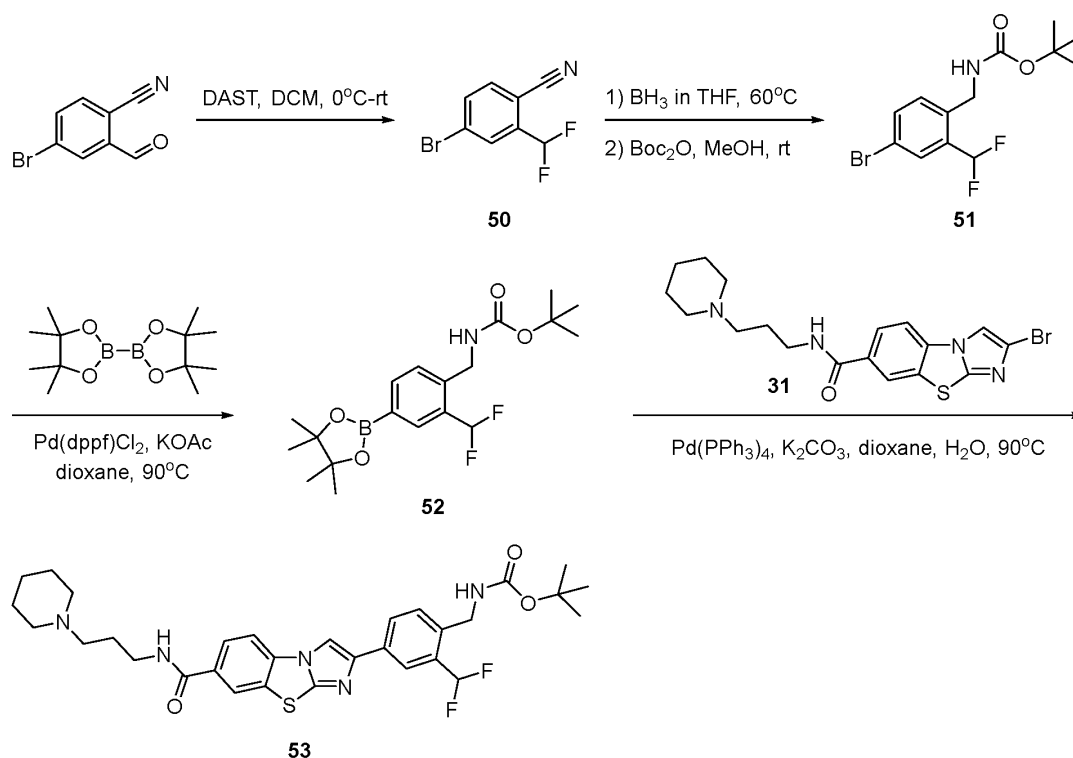
Scheme 38
