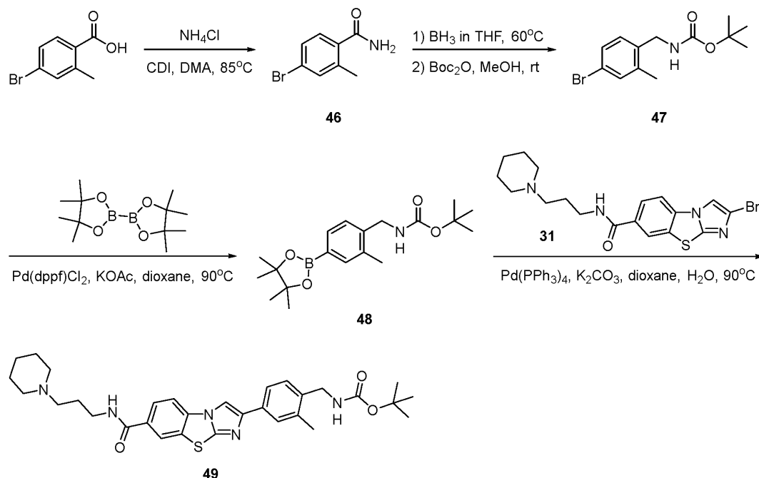
Scheme 37
