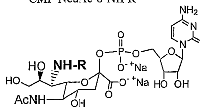
CMP-NeuAc-8-NH-R
