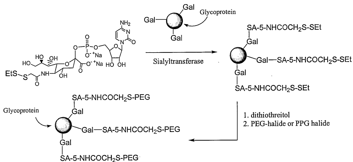
Scheme 4
