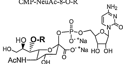
CMP-NeuAc-8-O-R
