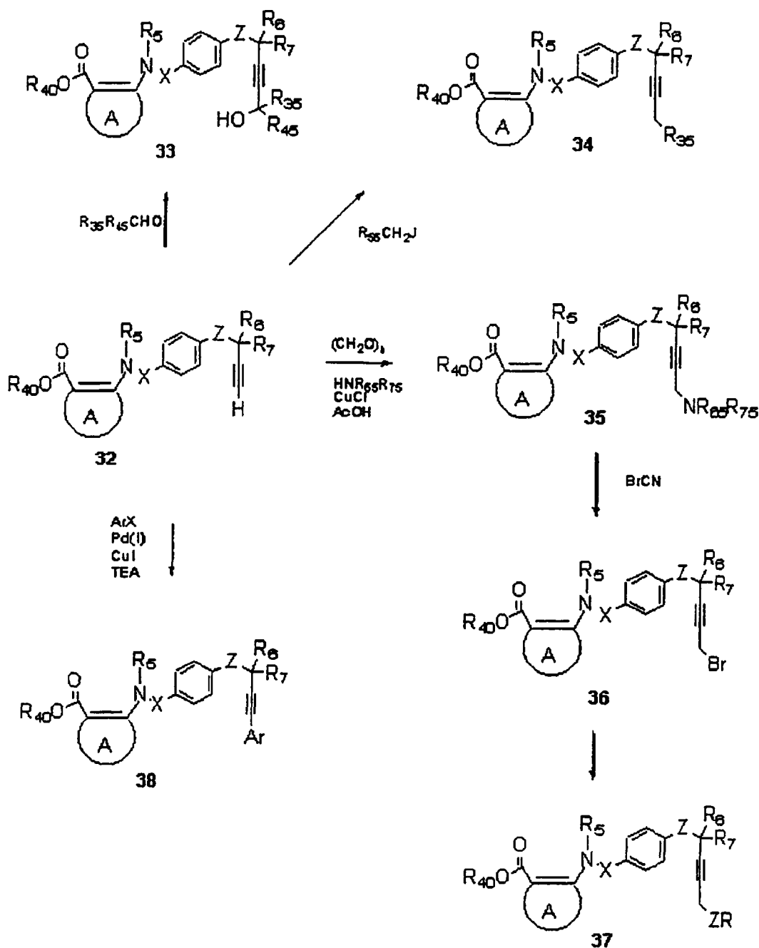
Scheme 9
