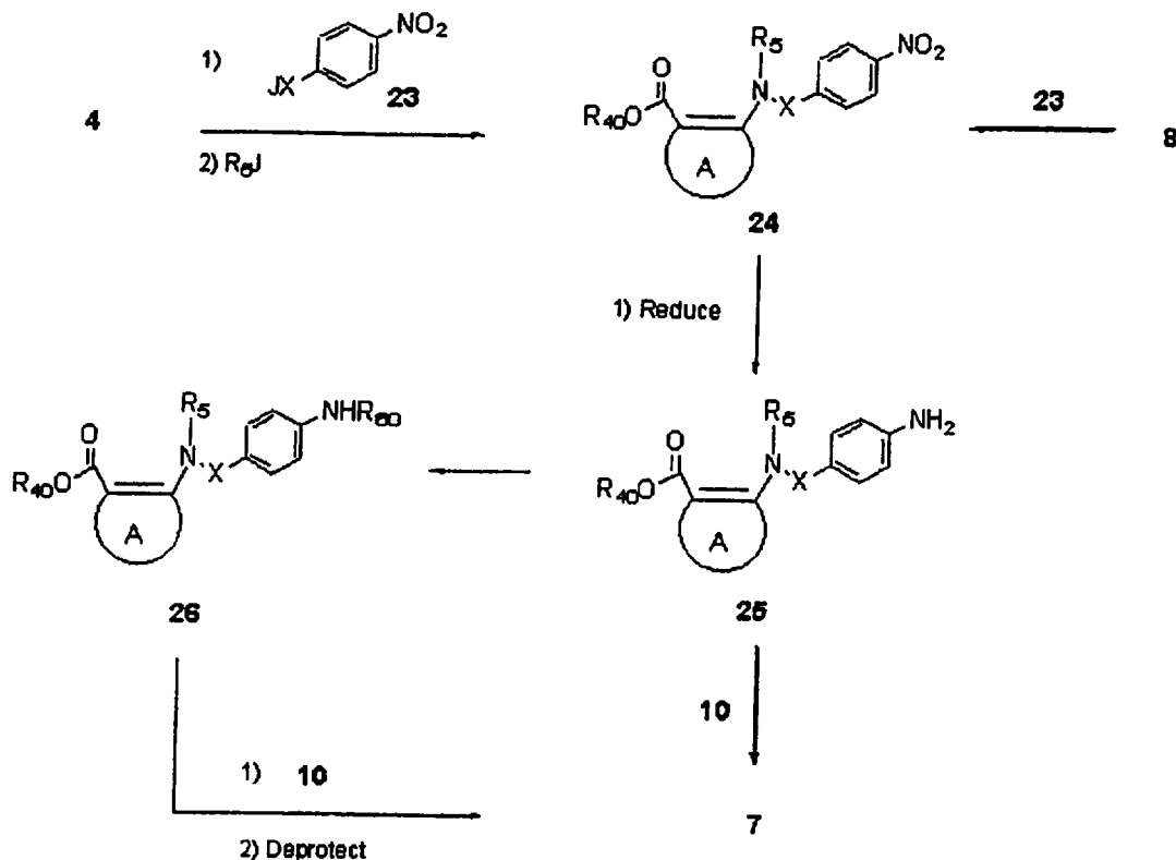
Scheme 6:
