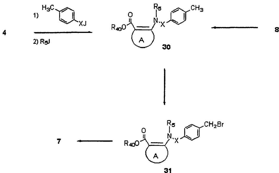
Scheme 8:
