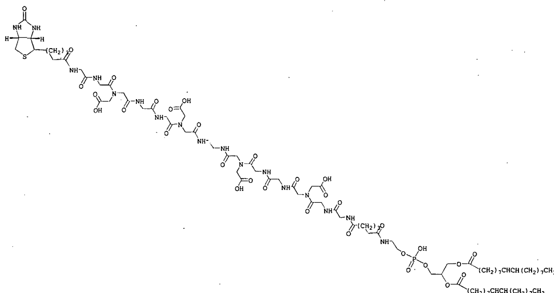
FSL-Biotin
