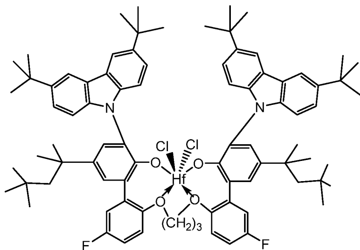
(7) ("Precatalyst 7")
