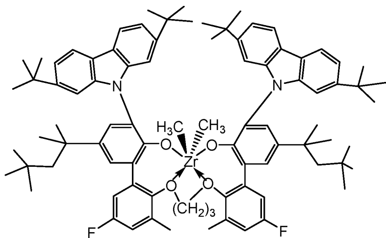
(6) ("Precatalyst 6")
