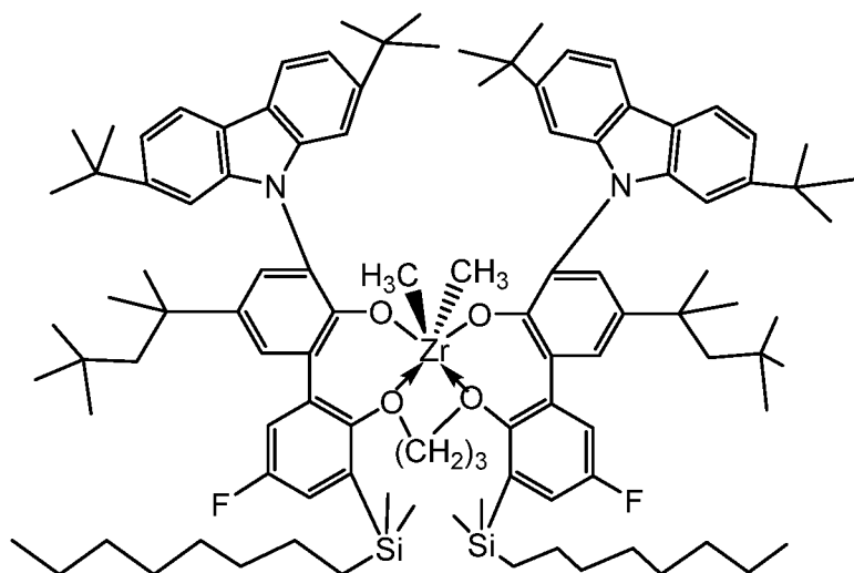
(8) ("Precatalyst 8");
