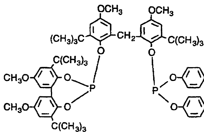
Ligand R
