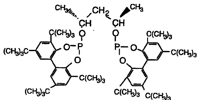
Ligand H
