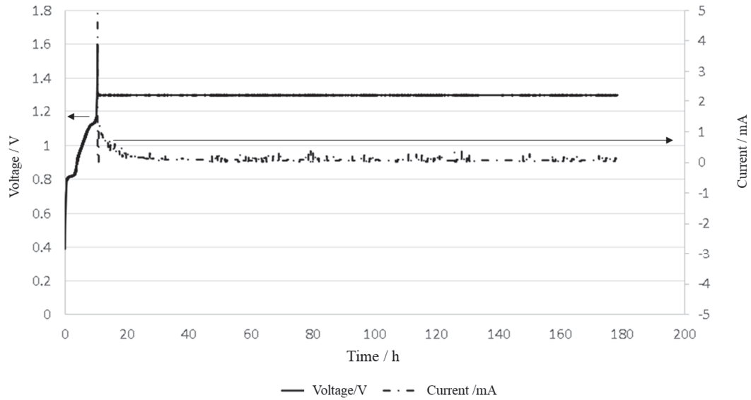
The current-voltage curve of Floating charge
