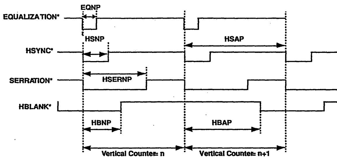
Horizontal Timing Waveforms—Interlaced Format
