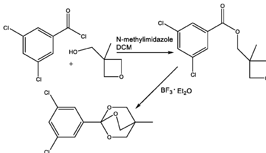
Reaction Scheme P2
