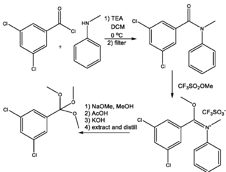
Reaction Scheme P1
