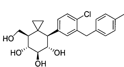
(4S,5S,6R,7R,8R)-4-(4-chloro-3-(4-ethylbenzyl)phenyl)-8-(hydroxymethyl)spiro[2.5]octane-5,6,7-triol
