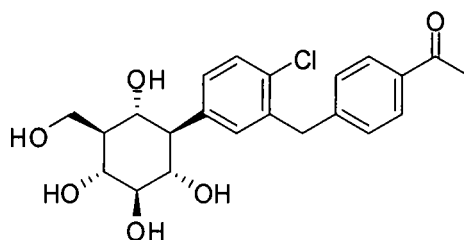
1-(4-(2-chloro-5-((1R,2S,3R,4R,5S,6R)-2,3,4,6-tetrahydroxy-5-(hydroxymethyl)cyclohexyl)benzyl)phenyl)ethanone
