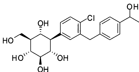
(1R,2R,3S,4R,5R,6S)-4-(4-chloro-3-(4-(1-hydroxyethyl)benzyl)phenyl)-6-(hydroxymethyl)cyclohexane-1,2,3,5-tetraol
