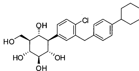
(1 R ,2 R ,3 S ,4 R ,5 R ,6 S )-4-(4-chloro-3-(4-cyclohexylbenzyl)phenyl)-6-(hydroxymethyl)cyclohexane-1,2,3,5-tetraol
