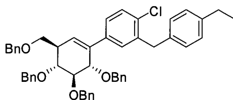
3 (R = Et)
