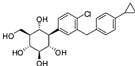
(1 R ,2 R ,3 S ,4 R ,5 R ,6 S )-4-(4-chloro-3-(4-cyclopropylbenzyl)phenyl)-6-(hydroxymethyl)cyclohexane-1,2,3,5-tetraol
