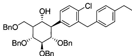
4 (R = Et)
