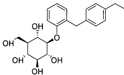
(1 R ,2 S ,3 R ,4 R ,5 S ,6 R )-4-(2-(4-ethylbenzyl)phenoxy)-6-(hydroxymethyl)cyclohexane-1,2,3,5-tetraol
