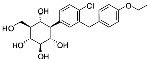
(1 R ,2 R ,3 S ,4 R ,5 R ,6 S )-4-(4-chloro-3-(4-ethoxybenzyl)phenyl)-6-(hydroxymethyl)cyclohexane-1,2,3,5-tetraol
