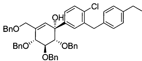
2 (R = Et)
