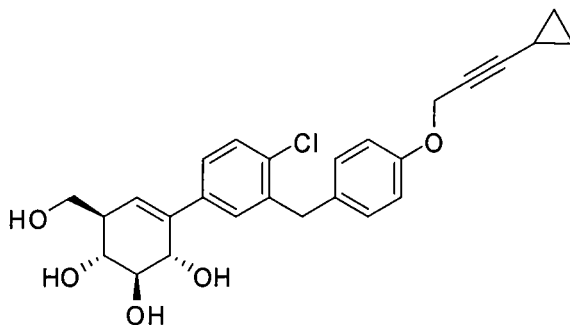
(1 R ,2 S ,3 S ,6 R )-4-(4-chloro-3-(4-(3-cyclopropylprop-2-ynyloxy)benzyl)phenyl)-6-(hydroxymethyl)cyclohex-4-ene-1,2,3-triol
