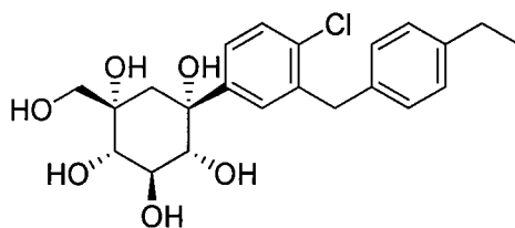
22 (R = Et)
