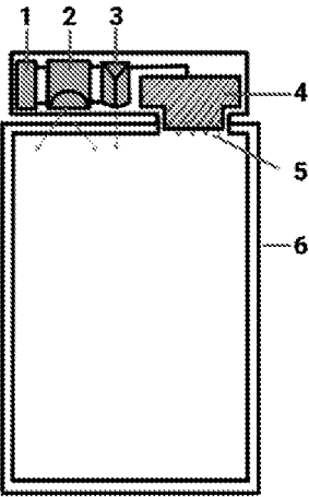
Figure 1: Battery Blast Prevention System (Without battery)
