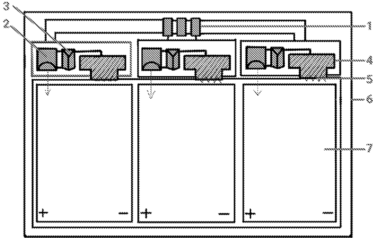
Figure 3: Multi-Battery Blast Prevention System
