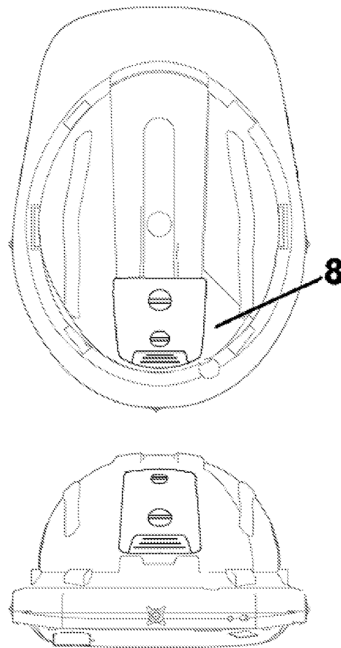
Figure 4: Battery Blast Prevention System installed inside the Smart Helmet
