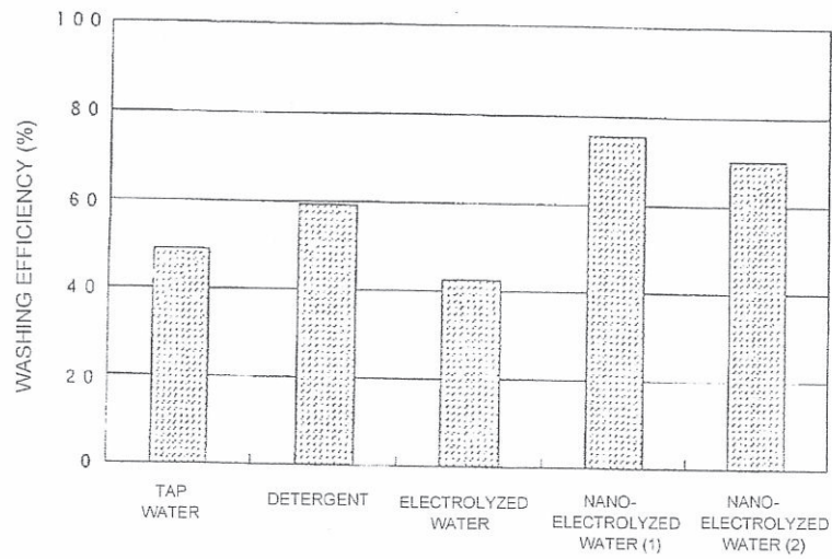
FIG. 5: WASHING RESULTS OF COCOA-SOILED FABRICS
