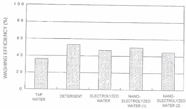
FIG. 3: WASHING RESULTS OF CARBON BLACK/MINERAL OIL-SOILED FABRICS
