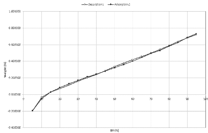
FIG. 4 Adsorption/Desorption Isotherm
