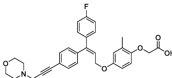
Compound I;
