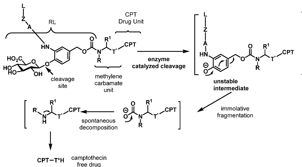
Scheme 1b:
