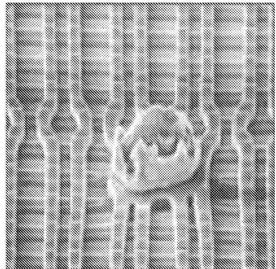
Defect Causing a Short A large, conducting defect shorts cut four wires in the circuit
