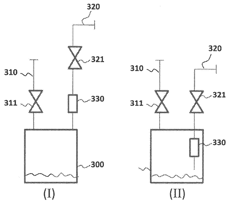
PACKAGE FOR Sb CONTAINING DOPANT MATERIALS
