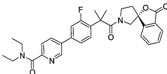
5-(4-{1,1-Dimethyl-2-oxo-2-[(1R)-3-oxo-1'H,3H-spiro[2-benzofuran-1,3'-pyrrolidin]-1'-yl]ethyl}-3-fluorophenyl)-N,N-diethylpyridine-2-carboxamide
