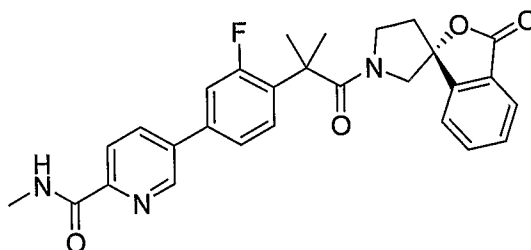
5-(4-{1,1-Dimethyl-2-oxo-2-[(1R)-3-oxo-1'H,3H-spiro[2-benzofuran-1,3'-pyrrolidin]-1'-yl]ethyl}-3-fluorophenyl)-N-methylpyridine-2-carboxamide
