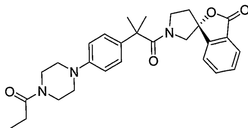
(1R)-1'-{2-Methyl-2-[4-(4-propionylpiperazin-1-yl)phenyl]propanoyl}-3H-spiro[2-benzofuran-1,3'-pyrrolidin]-3-one
