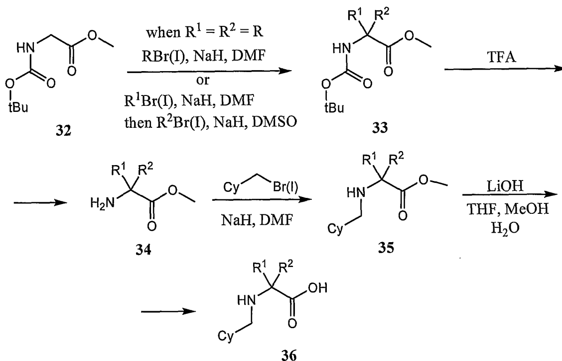
Scheme 9
