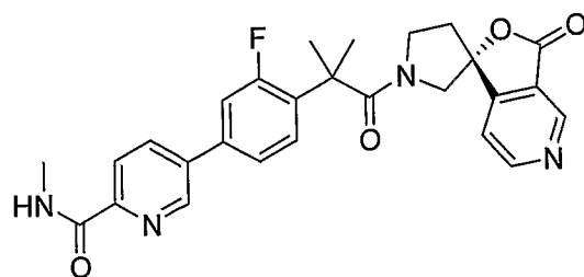
5-(4-{1,1-Dimethyl-2-oxo-2-[(1R)-3-oxo-1'H,3H-spiro[furo[3,4-c]pyridine-1,3'-pyrrolidin]-1'-yl]ethyl}-3-fluorophenyl)-N-methylpyridine-2-carboxamide
