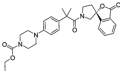
Ethyl 4-(4-{1,1-dimethyl-2-oxo-2-[(1R)-3-oxo-1'H,3H-spiro[2-benzofuran-1,3'-pyrrolidin]-1'-yl]ethyl}phenyl)piperazine-1-carboxylate
