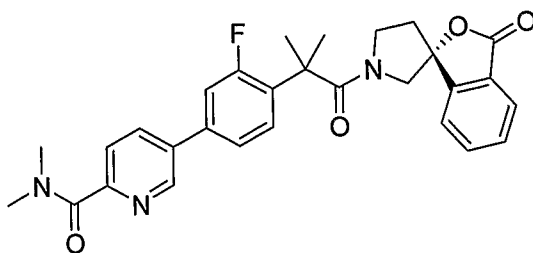
5-(4-{1,1-Dimethyl-2-oxo-2-[(1R)-3-oxo-1'H,3H-spiro[2-benzofuran-1,3'-pyrrolidin]-1'-yl]ethyl}-3-fluorophenyl)-N,N-dimethylpyridine-2-carboxamide
