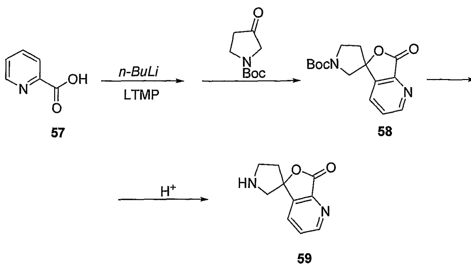
Scheme 17
