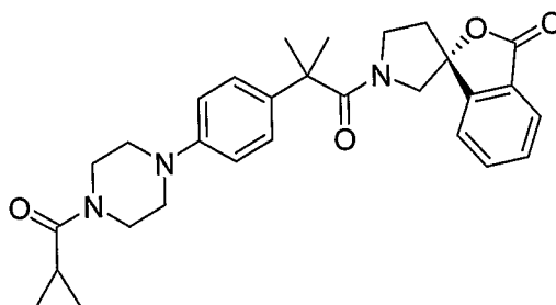
(1R)-1'-{2-[4-(4-Isobutyrylpiperazin-1-yl)phenyl]-2-methylpropanoyl}-3H-spiro[2-benzofuran-1,3'-pyrrolidin]-3-one
