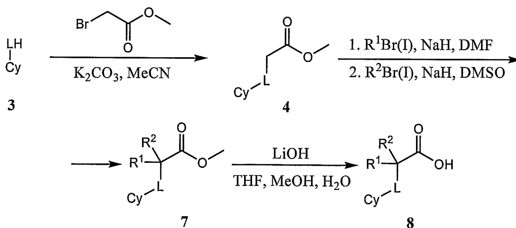
Scheme 3
