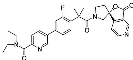
5-(4-{1,1-Dimethyl-2-oxo-2-[(1R)-3-oxo-1'H,3H-spiro[furo[3,4-c]pyridine-1,3'-pyrrolidin]-1'-yl]ethyl}-3-fluorophenyl)-N,N-diethylpyridine-2-carboxamide
