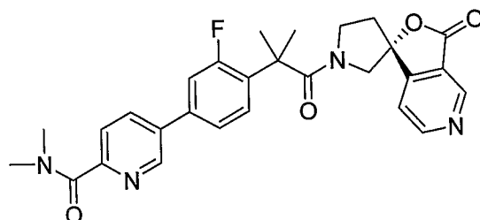
5-(4-{1,1-Dimethyl-2-oxo-2-[(1R)-3-oxo-1'H,3H-spiro[furo[3,4-c]pyridine-1,3'-pyrrolidin]-1'-yl]ethyl}-3-fluorophenyl)-N,N-dimethylpyridine-2-carboxamide
