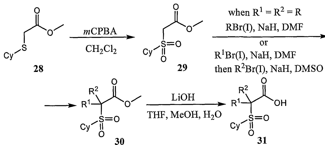
Scheme 8
