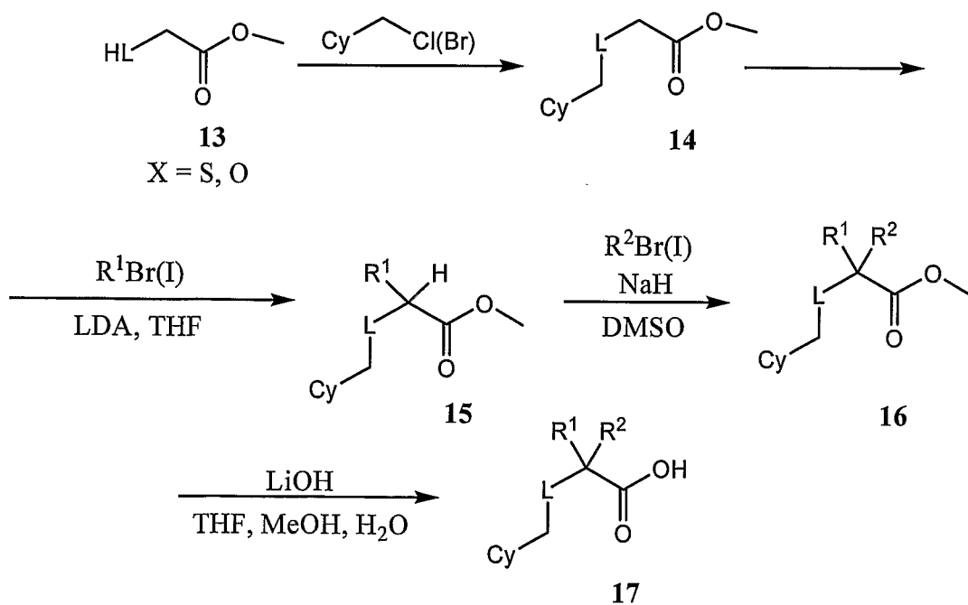
Scheme 5
