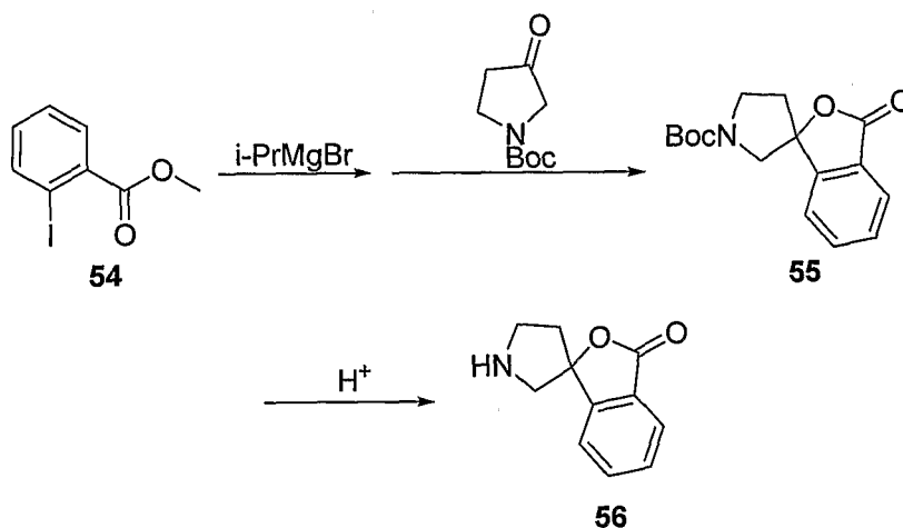
Scheme 16
