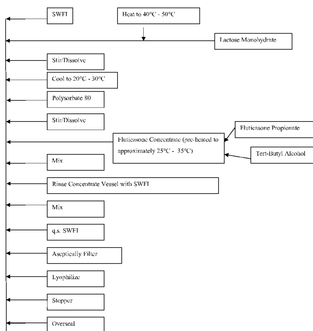
Figure 1. Fluticasone Propionate Lyophile Schematic
